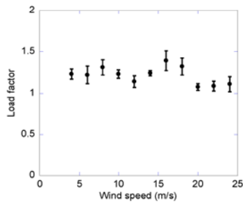
Fig. 4 Variation of load factor with mean wind speeds
