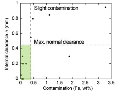
Fig. 5 Relationship of contamination and internal clearance of main bearings
