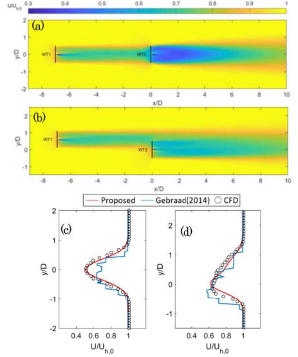
Figure 1. Contours and profiles (at x=4D ) of mean velocity in the wake of two wind turbines: (a), (c) for full overlap; (b), (d), for partial overlap.
