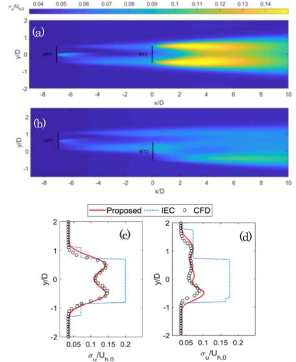
Figure 2. Contours and profiles (at x=4D ) of turbulence intensity in the wake of two wind turbines: (a), (c) for full overlap; (b), (d), for partial overlap.
