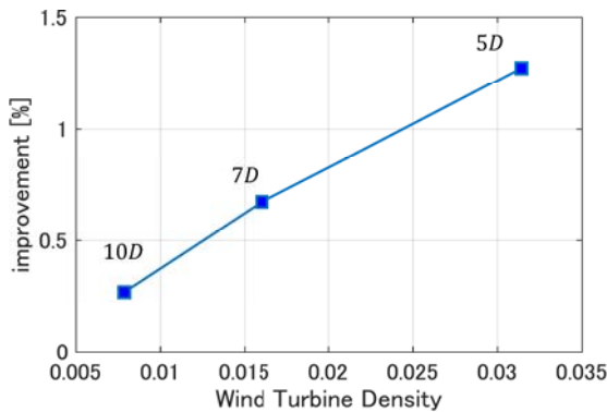
Figure 7. AEP improvements versus wind turbine density
