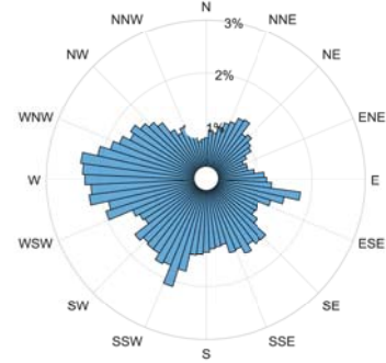
Figure 4. Wind direction distribution
