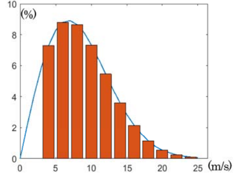
Figure 3. Rayleigh distribution with mean annual wind speed of 8.5m/s.
