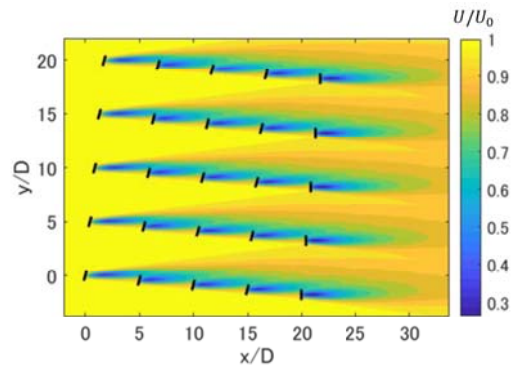
Figure 5. Example of optimized yaw offset and resulted wakes under certain wind speed and direction
