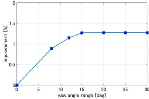
Figure 6. AEP improvements versus the yaw offset limit.
