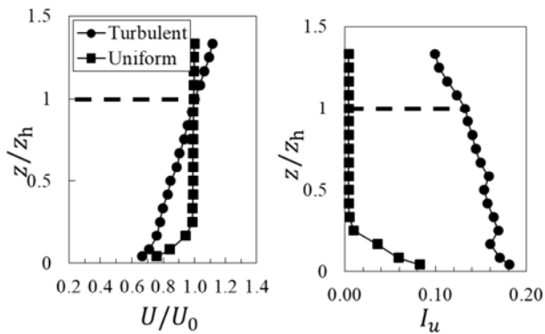
(a) Mean velocity (b) Turbulence intensity Fig. 2 Vertical profiles of mean velocity and turbulence intensity at the position of the nacelle model.
