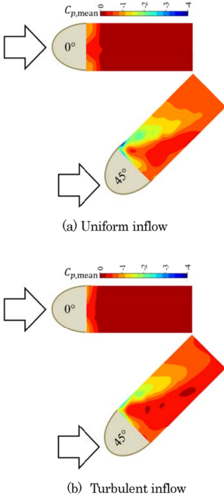
Fig. 4 Colormap of time-averaged pressure coefficient on the nacelle roof for 0° and 45° yaw angles.
