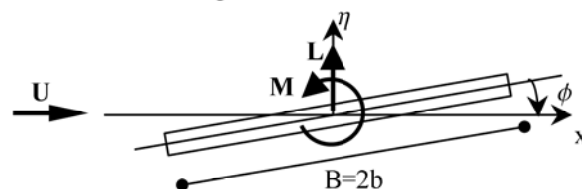
Fig. 2 Definition of motion and force components
