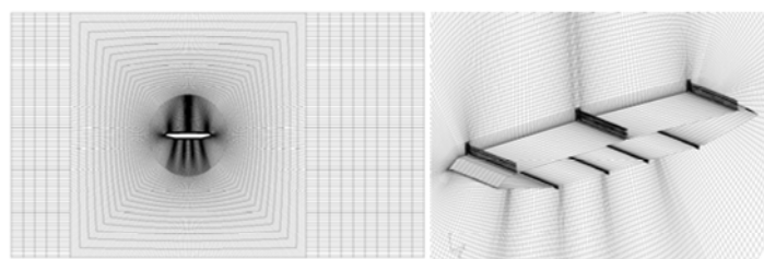
Fig. 1 Computational Domain of Nanjing Bridge cross-section and Rectangular cross-section
