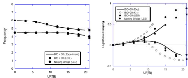
Figure 4 Eigen value loci of Rectangular cross section and Nanjing Bridge. M=1.96\text{kg/m} , I=4.9\times10^{-3}\text{Kg m}^2 , f_{\theta}=4.5\text{Hz} , f_{\phi}=6.0\text{Hz} , B/(2b)=0.15\text{m}
