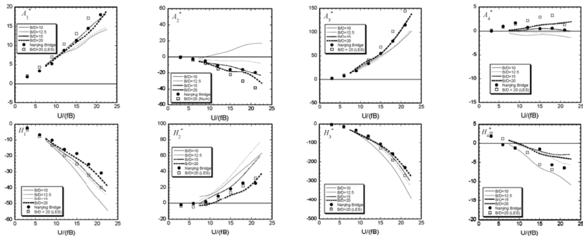
Fig. 3 Comparison of aerodynamic coefficients of Rectangular Section ( B/D=20 ) and Nanjing Bridge Section ( B/D=11.6 ) with the experimental results of different B/D ratios 3
