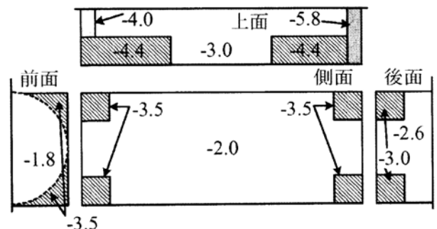
Fig.5 Schematic Distributions of Minimum Peak Pressure Coefficients for Panel Design Loads of Wind Turbine Nacelles
