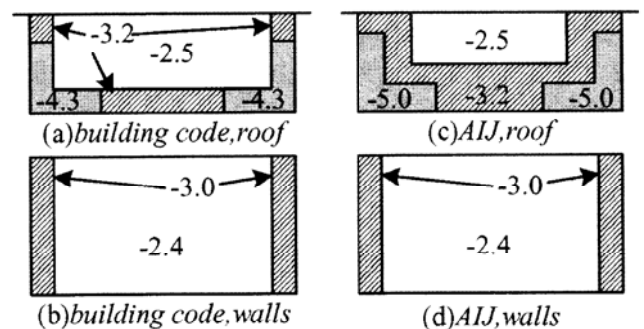
Fig.4 Minimum Peak Pressure Coefficients in Japan building code and AIJ Recommendations
