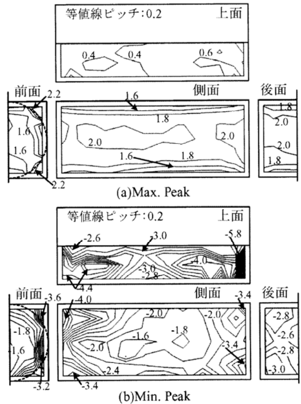
Figure.2 Peak Pressure Coefficient Distributions
