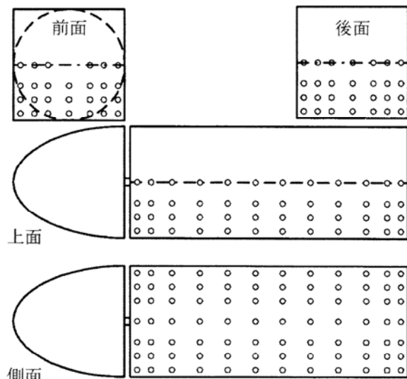
Figure.1 Pressure Measurement Points
