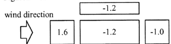
Fig.3 Pressure Coefficients for Nacelles in GL2003
