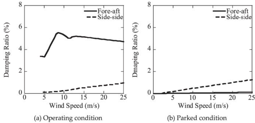
Fig. 3. Variation of aerodynamic damping ratio with wind speed.
