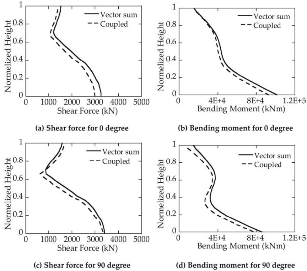
Fig. 23. Comparison of profiles of combined seismic and aerodynamic loads by the vector sum method and the coupled analysis approach for the parked condition.
