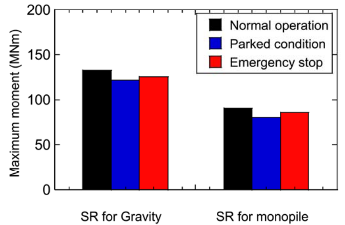
Fig. 16. The maximum tower base moments for different operational scenarios for wind turbine with different foundation types.
