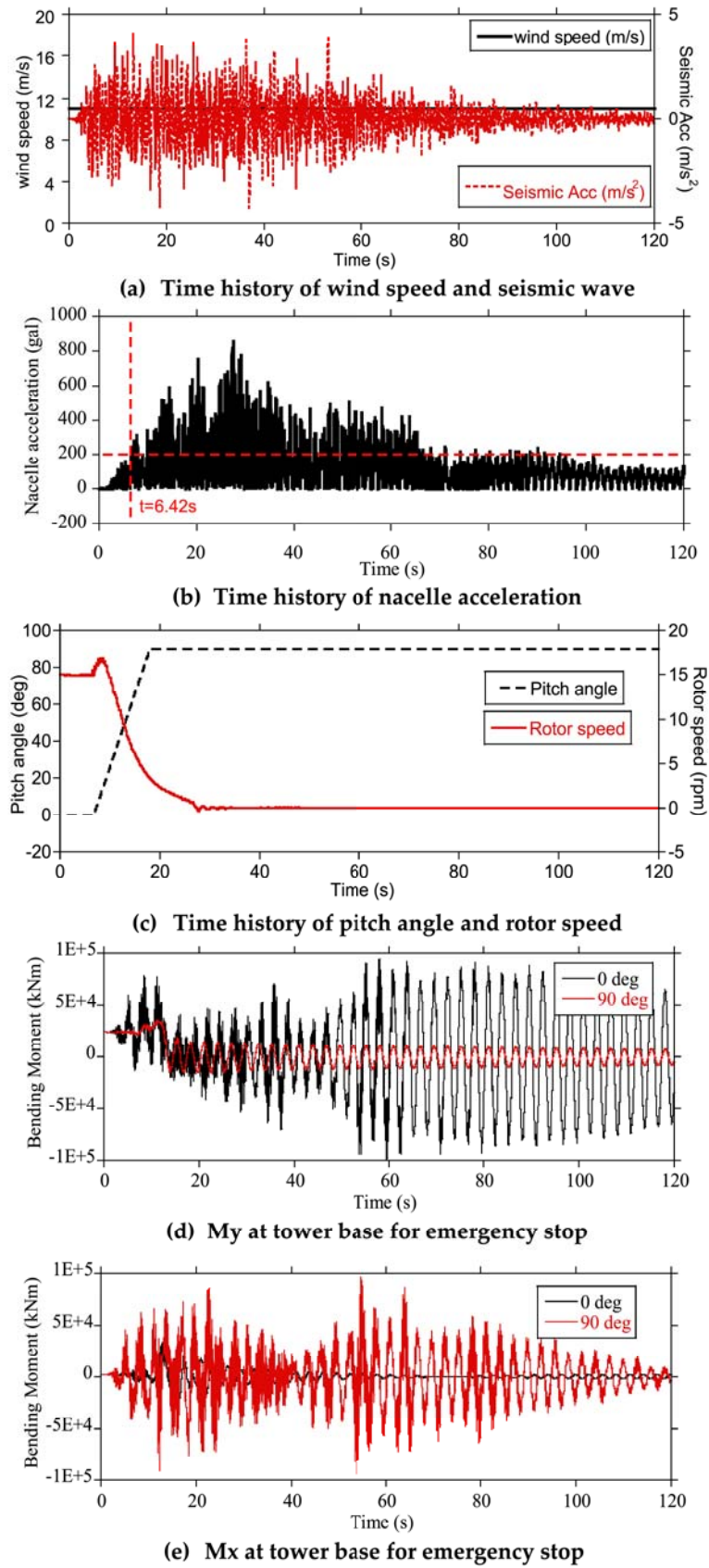
Fig. 11. Illustrations of various time histories during the emergency stop.
