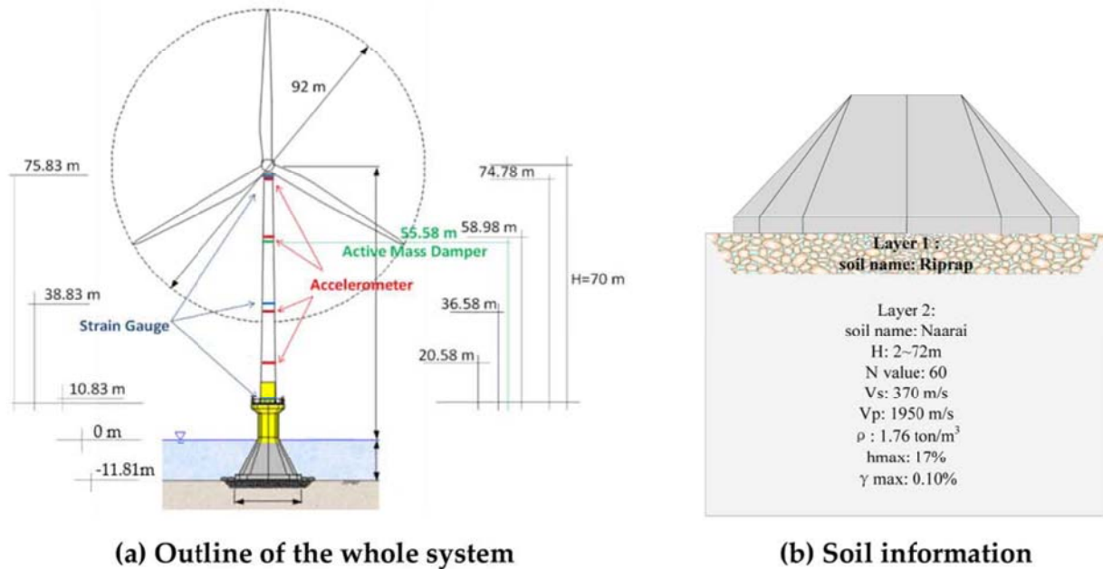
Fig. 1. Choshi wind power plant.
