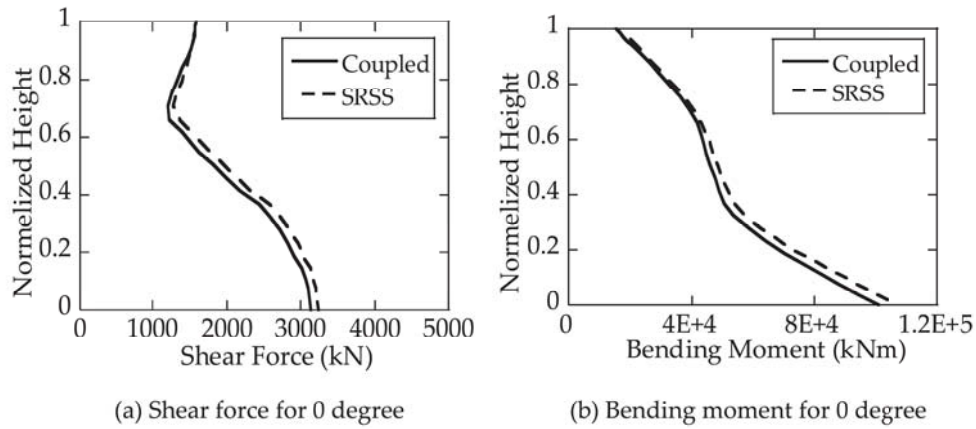
Fig. 21. Comparison of profiles of combined seismic and aerodynamic loads by the vector sum method and the coupled analysis approach for the emergency stop.
