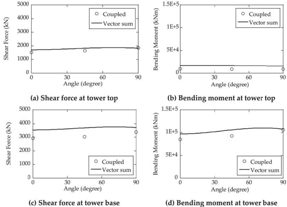
Fig. 19. Comparison of combined seismic and aerodynamic loads at tower top and base by the vector sum method and the coupled analysis approach for the normal operation.
