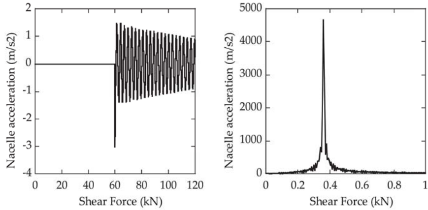
(a) Time-history of nacelle acceleration (b) Fourier spectrum of nacelle acceleration
