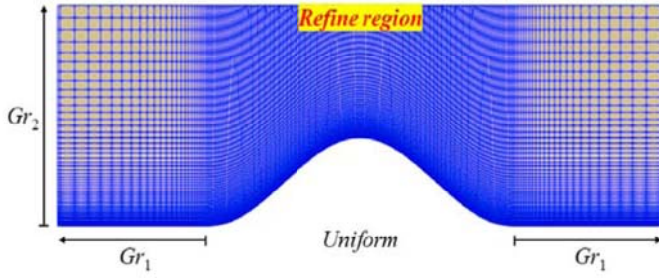
Fig. 10. Grid distributions around the three-dimensional hill.
