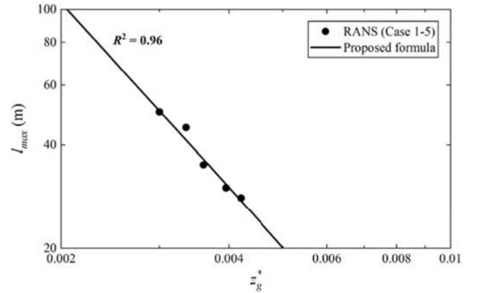
Fig. 8. Variation of the normalized gradient height z_g^* with maximum turbulence length scale l_{max} .
