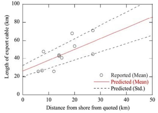
(b) Relationship between export cable length and distance from shore quoted for a distant landfall point
