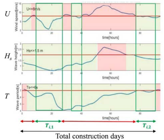
Fig. 7. Schematic of workability assessment.
