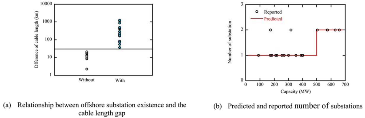
Fig. 16. Validation of offshore substation model.
