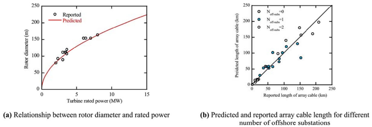
Fig. 17. Validation of array cable length.
