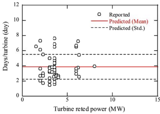
(a) Installation days for one turbine.
