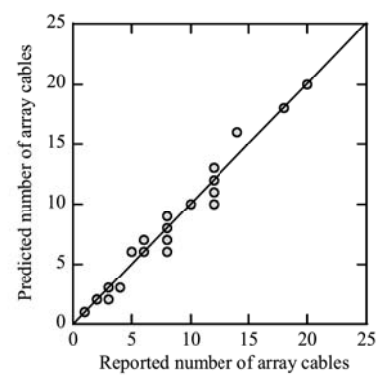
(b) Predicted and recorded array cable number
