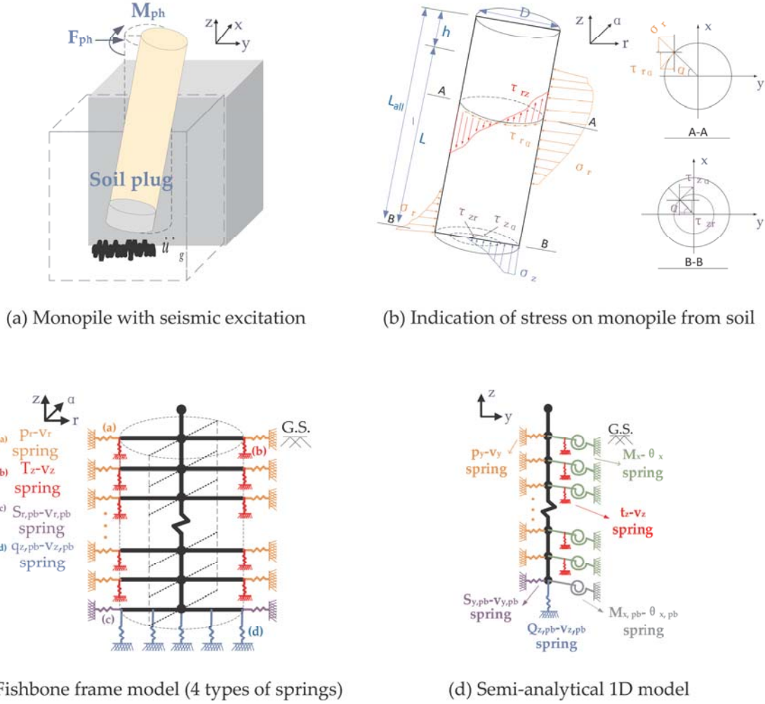
Fig. 1. Monopile foundation and its dynamic semi-analytical model.
