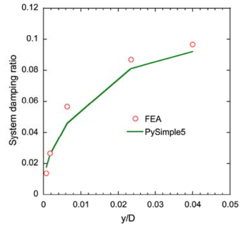
Fig. A4. Comparison of foundation damping ratios calculated by FEA and BNWF model with PySimple5.
