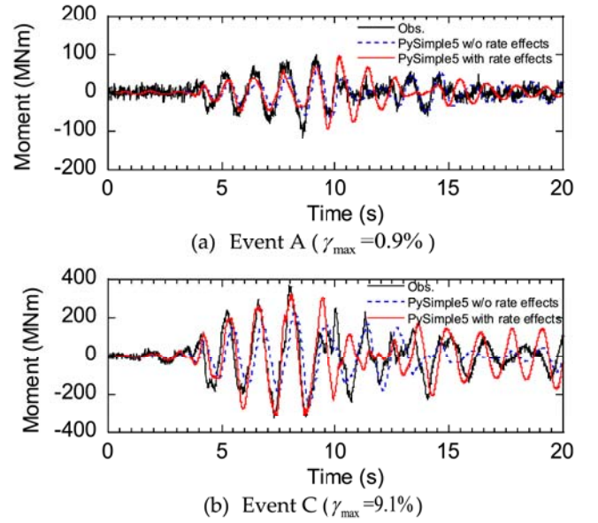
Fig. 13. Comparisons of measured and predicted bending moment time histories at depth of 0.76 m.
