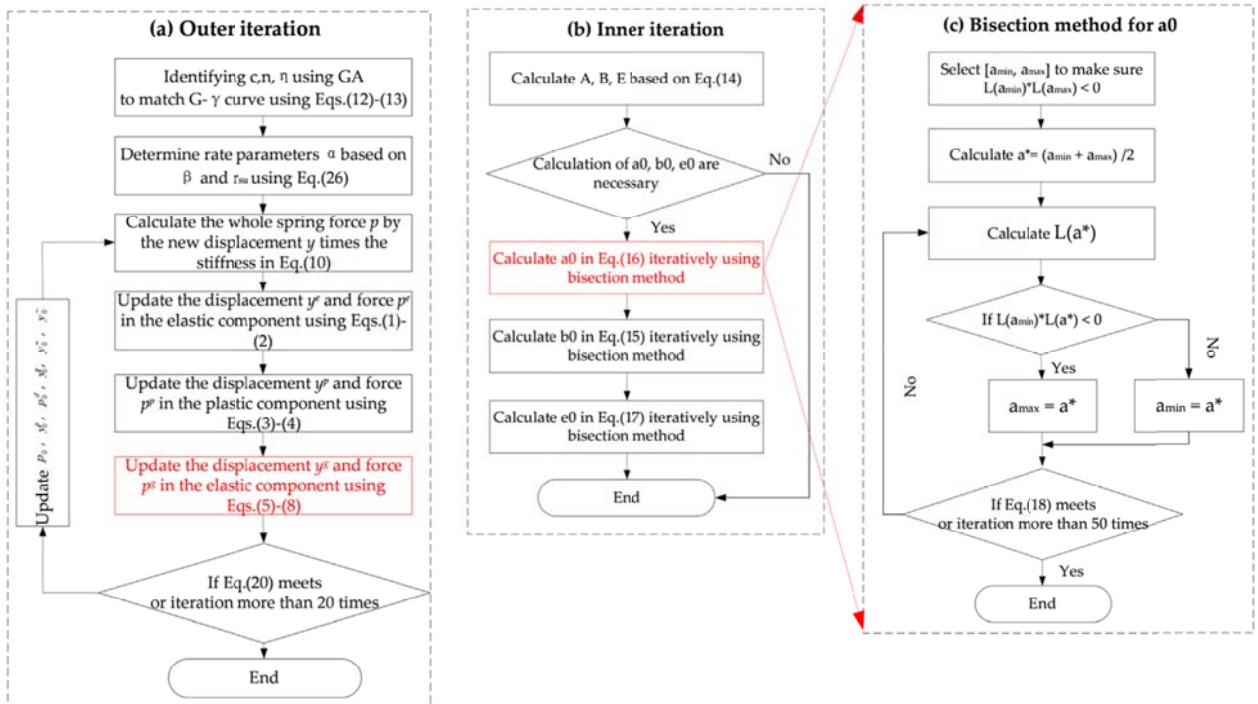
Fig. 3. Flow chart for determining parameters in PySimple5.
