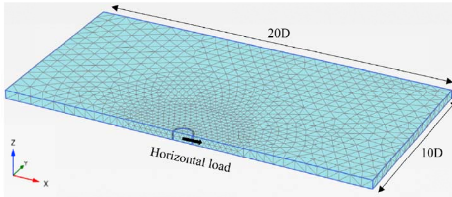
Fig. A1. Three-dimensional finite element model corresponding to single p-y element (After, Zhang et al. 2021).
