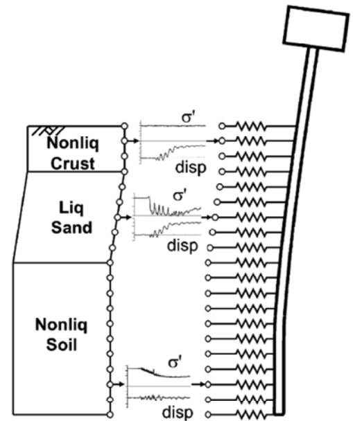
Fig. 4. Schematic of ground motion and mean effective stress from site response analysis input to free ends of PyLiq1 elements (Brandenburg et al., 2013).
