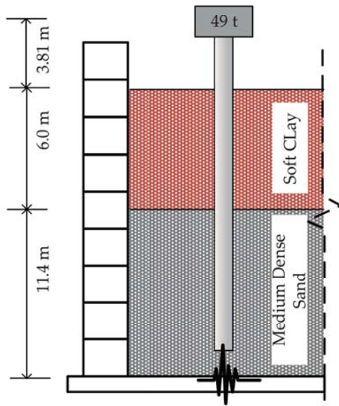
Fig. 7. Schematic of CSP5 centrifuge tests (after Wilson, 1998).
