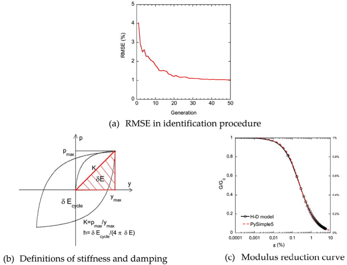
Fig. 2. Example of PySimple5 backbone curve using parameters given in Table 1 and modulus reduction curve derived from PySimple5.
