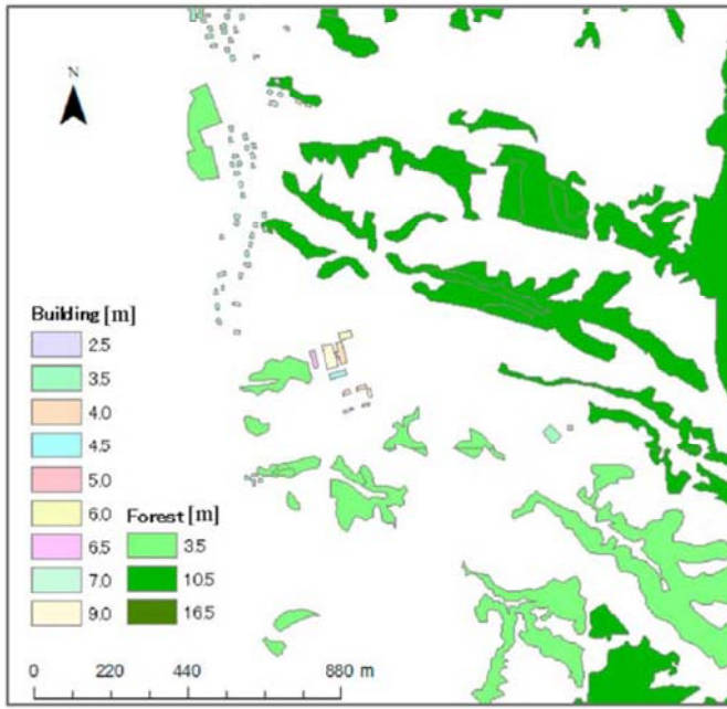
Fig. 14. Digital map of buildings and forests in the wind farm. The values of different legend represent the height of canopies.
