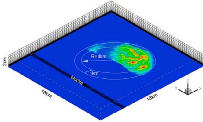
Fig. 13. Configuration of computational domain with terrain topography.
