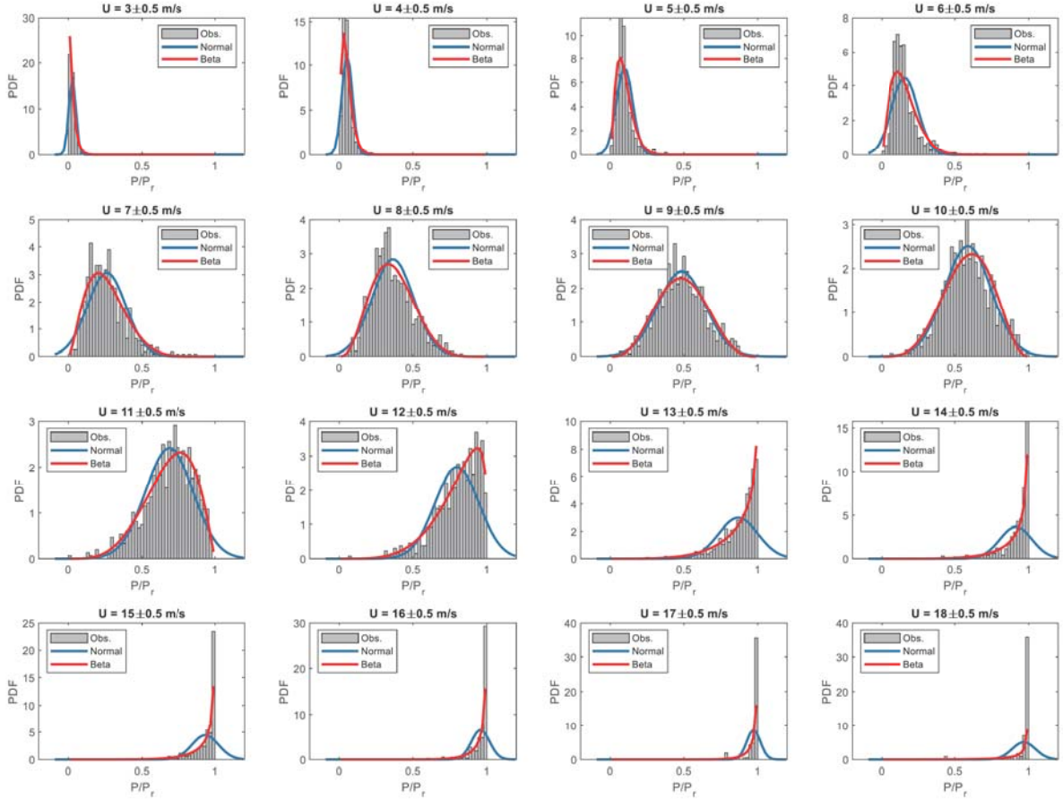
Fig. 8. Probability density distribution of power outputs within each wind speed bin for WT1.
