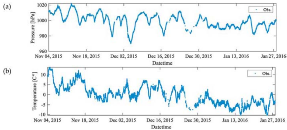
Fig. 5. Time series of 10-minutue averaged (a) atmospheric pressure and (b) temperature measured at the height of 75 m by Met-mast No.1.
