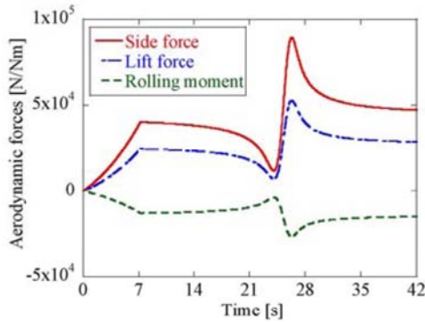
Fig. 13. Tornado-induced aerodynamic forces ( V_{Max,T} = 41\text{m/s} , R_{Max} = 30\text{m} , V_r = 100\text{km/h} ).
