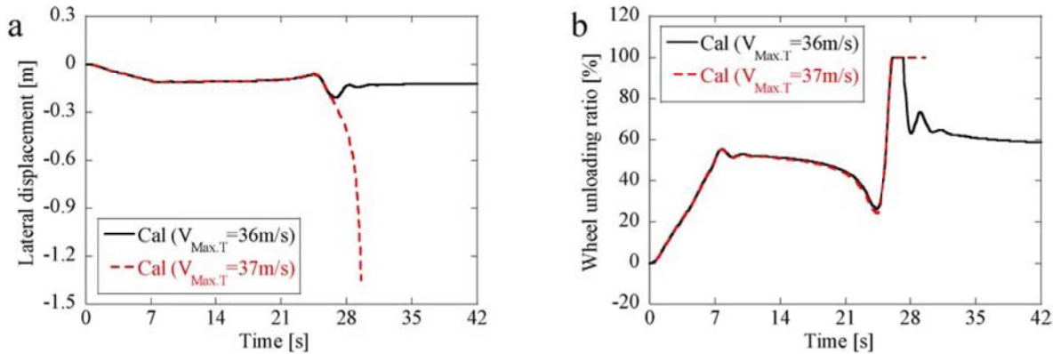
Fig. 14. Predicted dynamic responses of the limited express train in tornado winds ( R_{Max} = 30\text{m} ): (a) lateral displacement of the gravity center of car body and (b) wheel unloading ratio.
