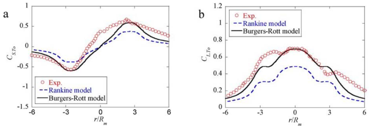
Fig. 11. Tornado-induced aerodynamic force coefficients: (a) side force coefficient; (b) lift force coefficient.
