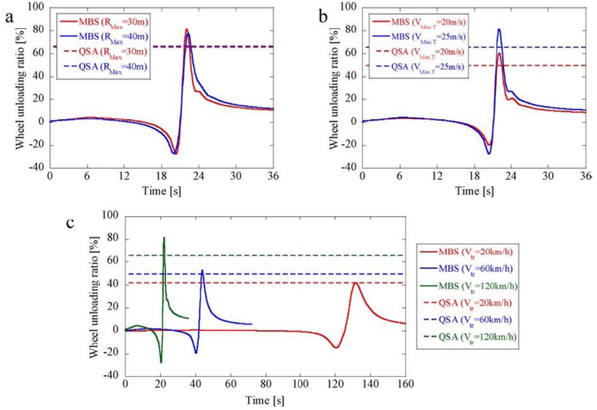
Fig. 18. Variations of wheel unloading ratio with: (a) core radius ( V_{Max,T} = 25\text{m/s} , V_{tr} = 120\text{km/h} ); (b) maximum tangential wind speed ( R_{Max} = 30\text{m} , V_{tr} = 120\text{km/h} ); (c) train velocity ( R_{Max} = 30\text{m} , V_{Max,T} = 25\text{m/s} )
