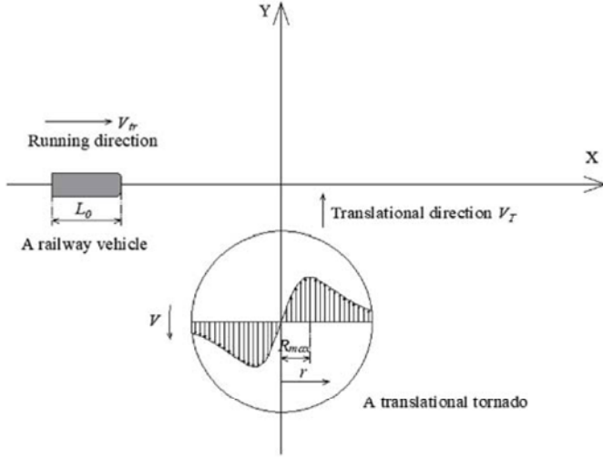
Fig. 1. A schematic of a tornado hitting a railway vehicle.
