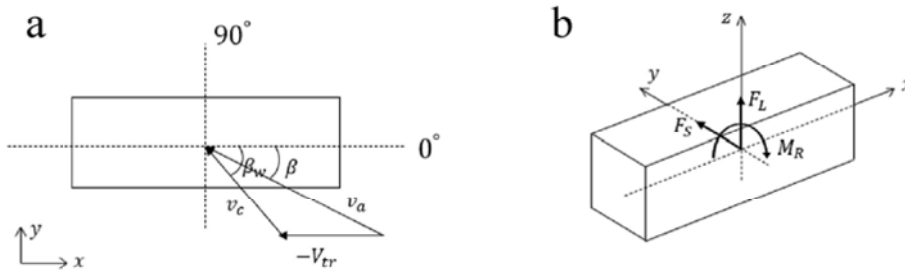
Fig. 2. Coordinate systems for: (a) wind direction; (b) aerodynamic forces direction.
