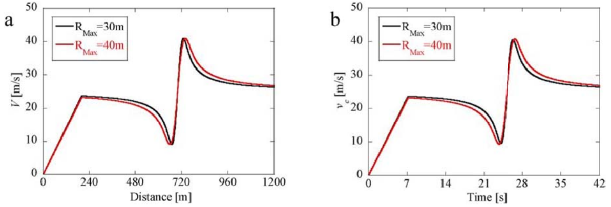
Fig. 12. The tangential velocity: (a) distributed along the track in spatial domain; (b) at the vehicle center in time domain ( V_{Max,T} = 41\text{m/s} , V_r = 100\text{km/h} ).
