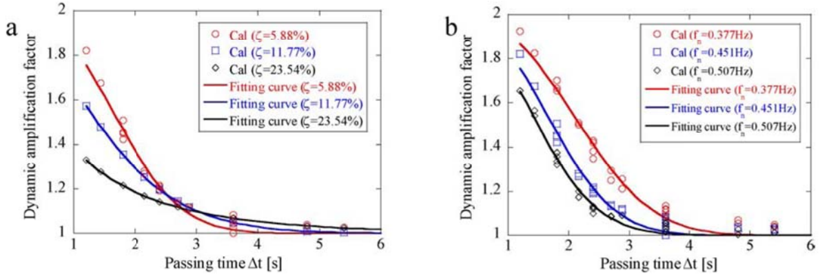
Fig. 20. Variations of DAF with the passing time as functions of (a) damping ratio ( f_n = 0.451\text{Hz} ) and (b) natural frequency ( \zeta = 5.88\% ).
