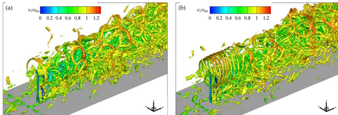
Fig. 15. Vortex structure in the wake flow of wind turbine: (a) ADM-R, (b) ALM.
