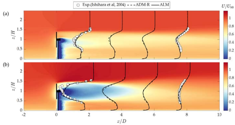
Fig. 13. Contours and profiles of mean velocity in the vertical x-z plane through the center of the rotor of laboratory-scale wind turbine: (a) C_t = 0.37 , (b) C_t = 0.81 .
