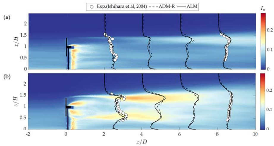
Fig. 14. Contours and profiles of turbulence intensity the vertical x-z plane through the center of the rotor of laboratory-scale wind turbine in the wind tunnel test: (a) C_t = 0.37 , (b) C_t = 0.81 .
