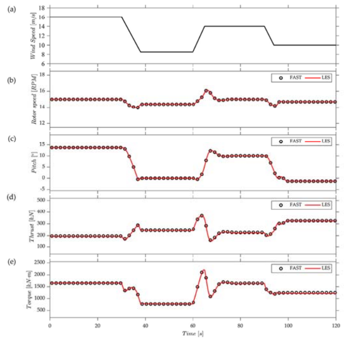
Fig. 9. Time series of (a) benchmark inflow wind speed, control signal of (b) rotor speed and (c) pitch angle, (d) rotor thrust force, and (e) rotor torque force.
