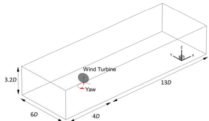
Fig. 8. Bird's eye view of the computational domain: wind turbine control simulation for a utility-scale Choshi-2.4 MW wind turbine under uniform inflow.
