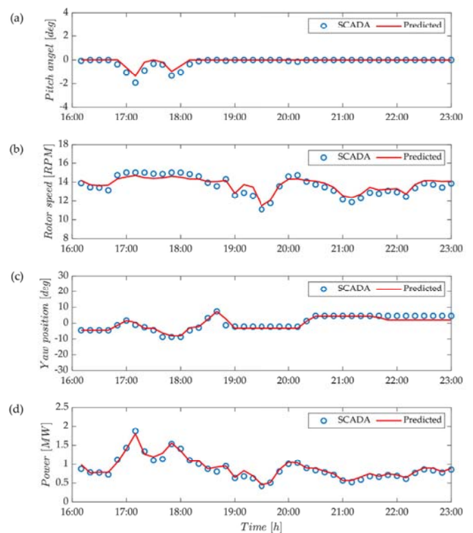
Fig. 20. Comparison of the time series of 10-minute averaged (a) pitch angle, (b) rotor speed, (c) yaw position and (d) Power production between SCADA data and results predicted by LES. The time series of yaw position has subtracted the mean wind direction during the 7 h.
