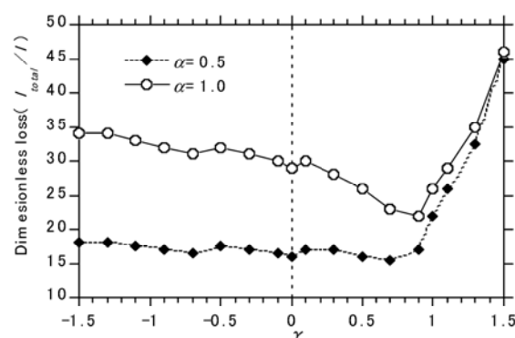
Figure 9. Difference in dimensionless loss due to difference in \gamma .
