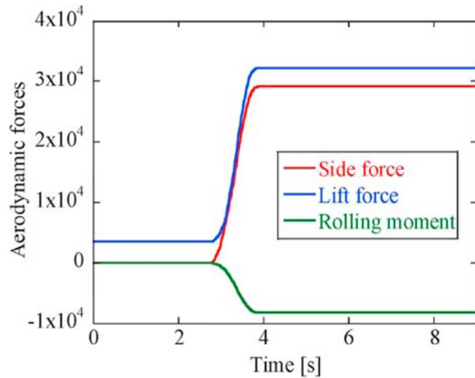
Fig. 16. Aerodynamic forces caused by tunnel exit winds ( U_0 = 20m/s , L = 20m , V_r = 120km/h ).
