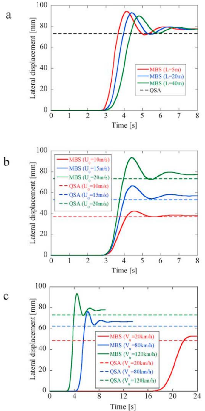
Fig. 17. Variations of lateral displacement of center of gravity of car body with: (a) gust duration ( U_0 = 20m/s , V_r = 120km/h ); (b) gust amplitude ( L = 20m , V_r = 120km/h ); (c) train velocity ( L = 20m , U_0 = 20m/s ).
