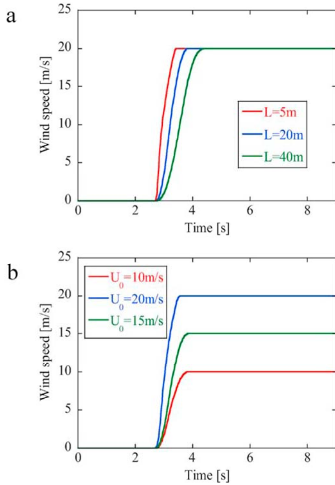
Fig. 15. Variations of tunnel exit winds at vehicle center in time domain ( V_r = 120km/h ): (a) with gust duration; (b) with gust amplitude.
