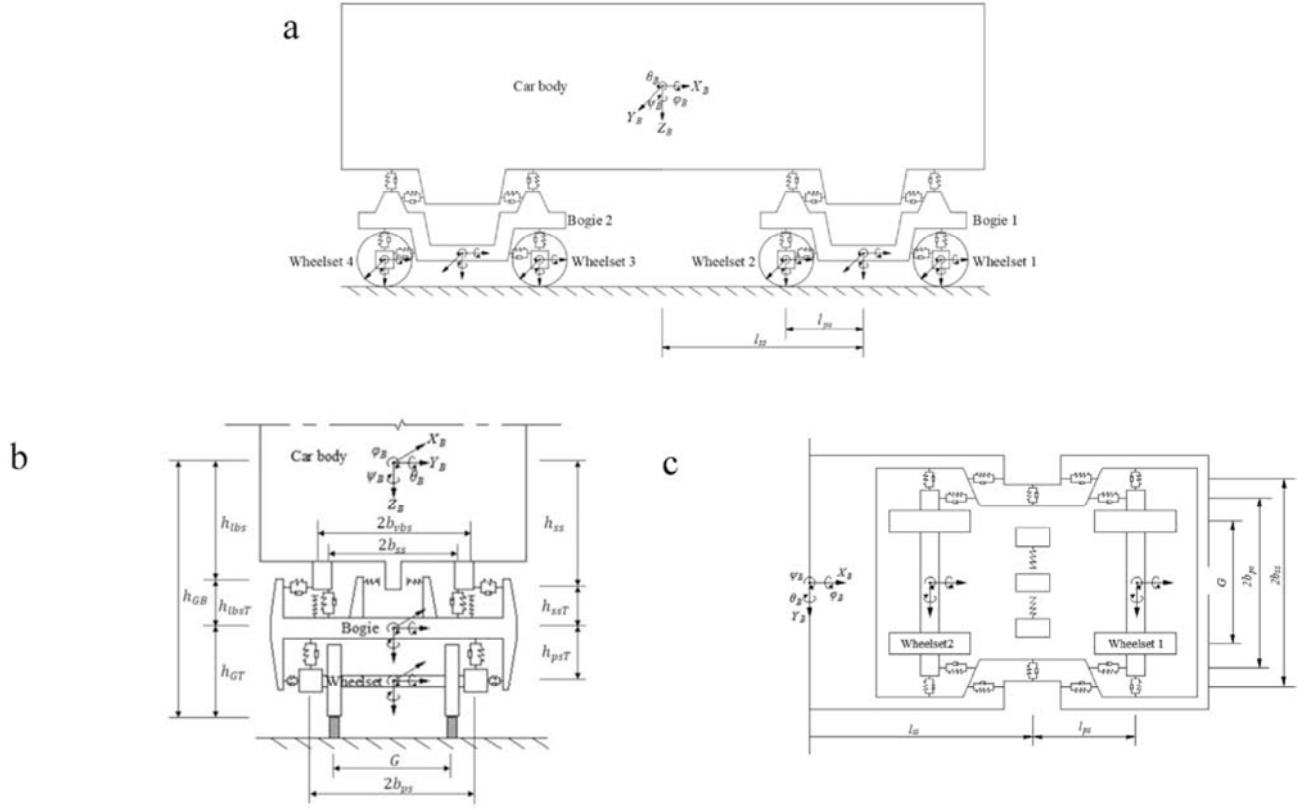
Fig. 5. A full vehicle model used in this study: (a) side view; (b) end view; (c) top view.
