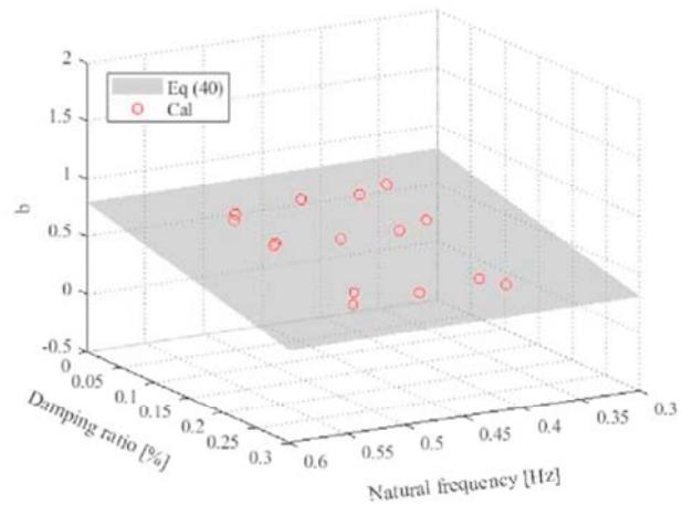
Fig. 20. Variations of: (a) a(f_n, \zeta) and (b) b(f_n, \zeta) with the damping ratio and natural frequency.
