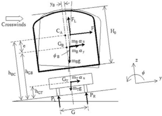
Fig. 4. A two-dimensional vehicle model used in the quasi-static analysis.
