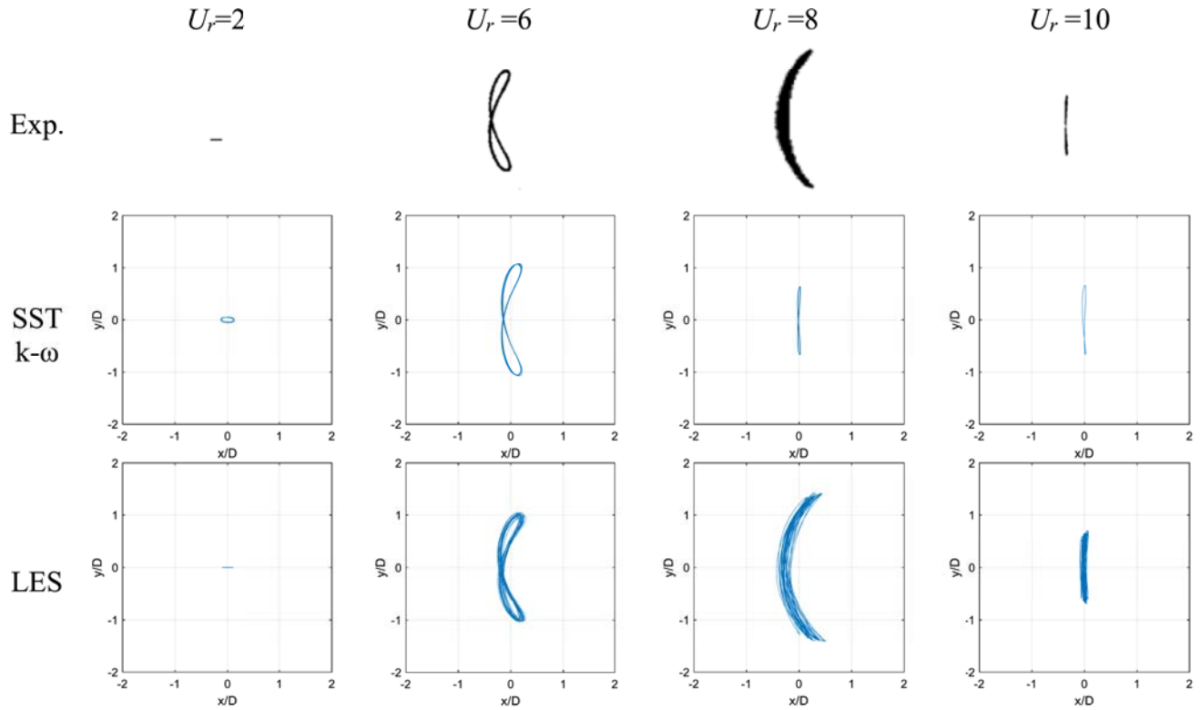
Fig. 5. Vibration trajectory of circular cylinder with 2DOF linear system.
