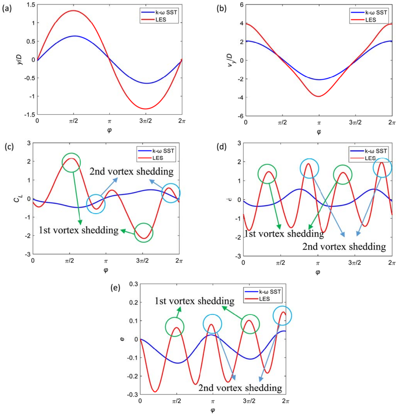
Fig. 11. Averaged (a) transverse displacement, (b) transverse velocity, (c) lift coefficient, (d) energy transfer rate and (e) energy transfer in one cycle of oscillation at U_f = 8 for the circular cylinder with 2DOF linear system.
