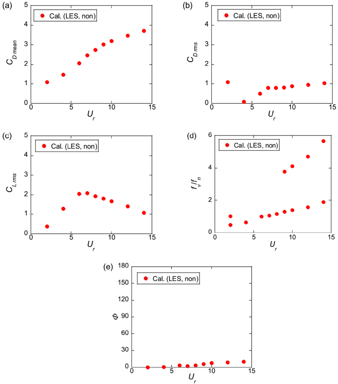
Fig. 13. Variation of (a) mean drag coefficients C_{D\ mean} , (b) fluctuating drag coefficients C_{D\ rms} , (c) fluctuating lift coefficients C_{L\ rms} , (d) non-dimensional vortex shedding frequency f_v/f_n and (e) phase angle \Phi between lift force and transverse displacement with U_r for the circular cylinder with 2DOF nonlinear system.
