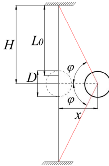
Fig. A.1. Schematic of geometrical nonlinear system.
