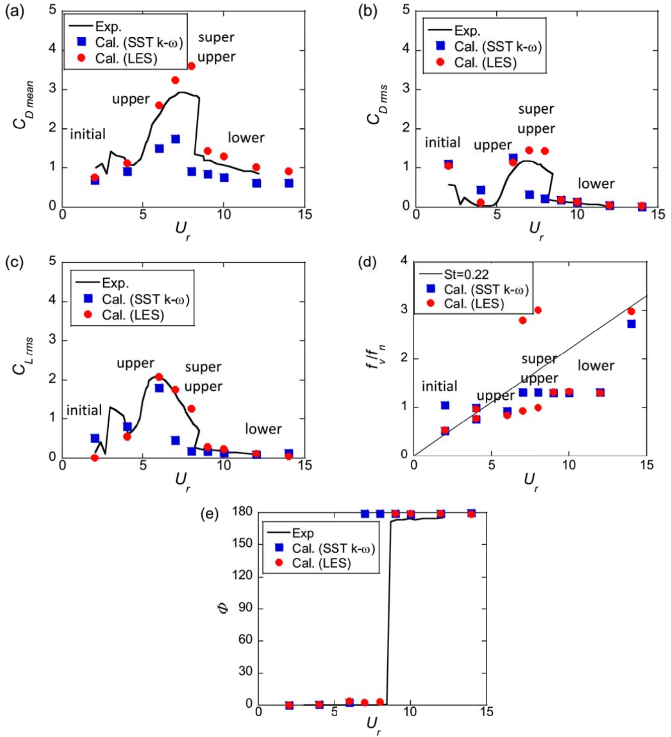
Fig. 4. Variation of (a) mean drag coefficients C_{D\text{ mean}} , (b) fluctuating drag coefficients C_{D\text{ rms}} , (c) fluctuating lift coefficients C_{L\text{ rms}} , (d) non-dimensional vortex shedding frequency f_v/f_n and (e) phase angle \phi between lift force and transverse displacement with U_r for the circular cylinder with 2DOF linear system.
