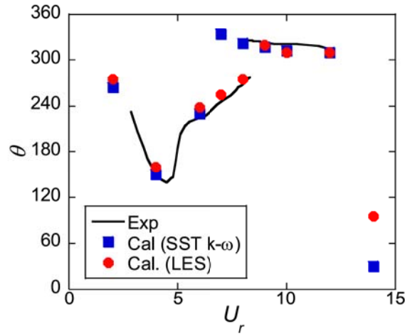
Fig. 6. Phase angles between streamwise and transverse motion.
