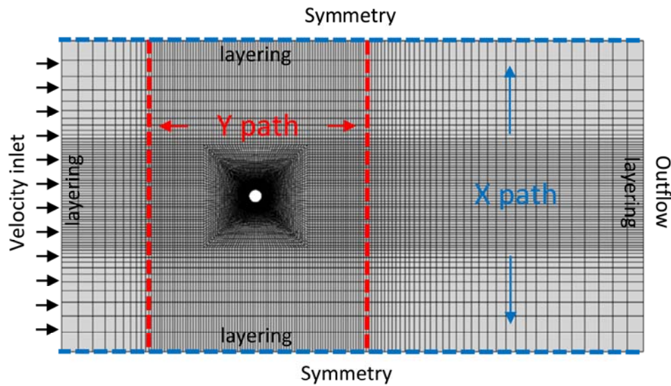
Fig. 2. Numerical mesh and boundary conditions.
