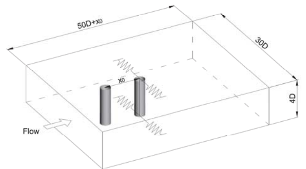
Fig. 1. Overview of computational domain.
