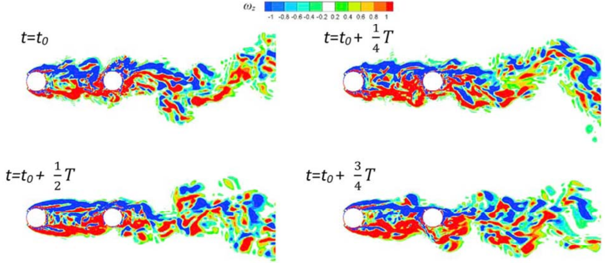
Fig. 30. Vorticity around tandem circular cylinders with helical wires for m^* = 200 and x_0/D = 4 at U_r = 100 .
