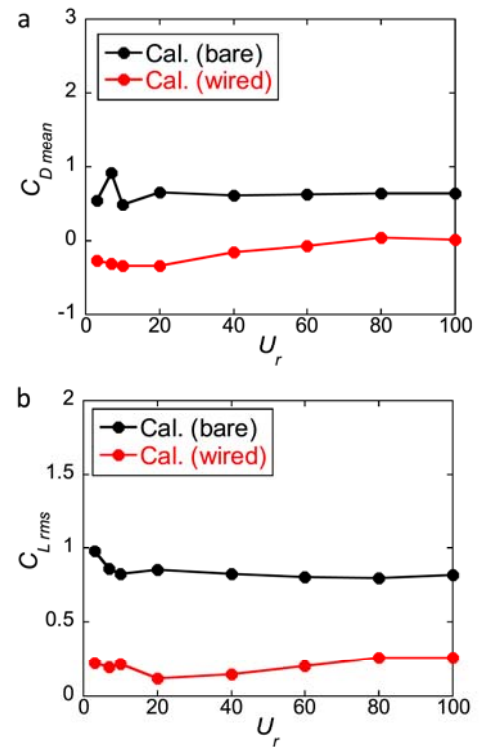
Fig. 29. Comparison of (a) mean drag coefficients and (b) fluctuating lift coefficients of the downstream cylinders with and without helical wires for m^* = 200 and x_0/D = 4 .
