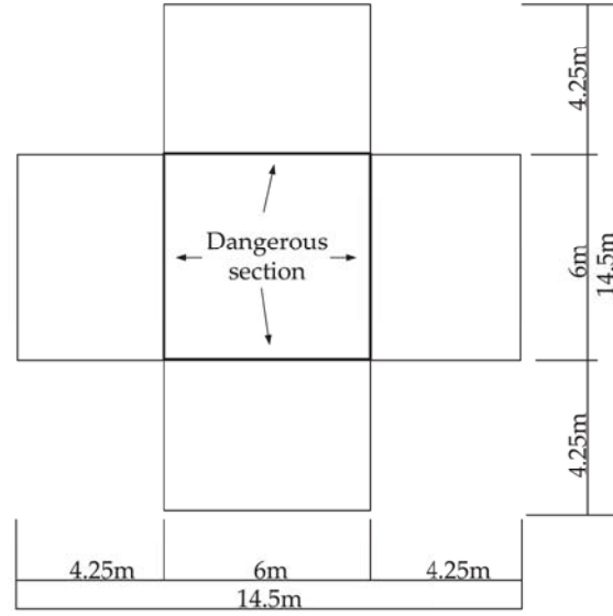
(b) Top view of shallow foundation
