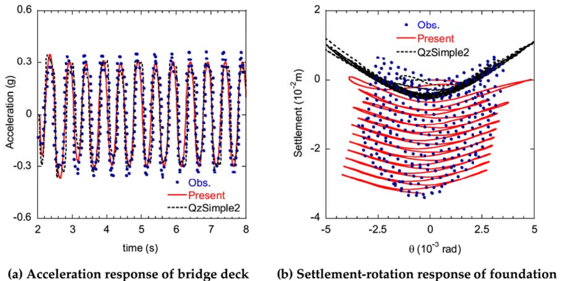
Fig. 6. Comparison of the responses under the base excitation of a 12-cycle 2-Hz sine pulse with a 0.50 g acceleration amplitude.
