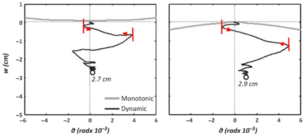
(b) Settlement-rotation response: Large foundation (left) and Medium foundation (right)
