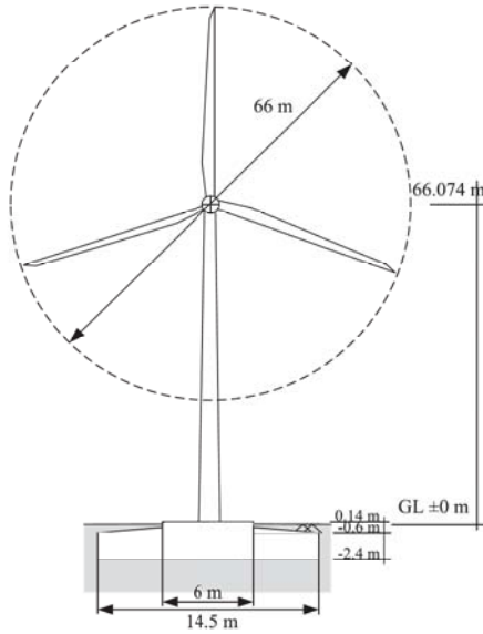
(a) Outline of the whole system
