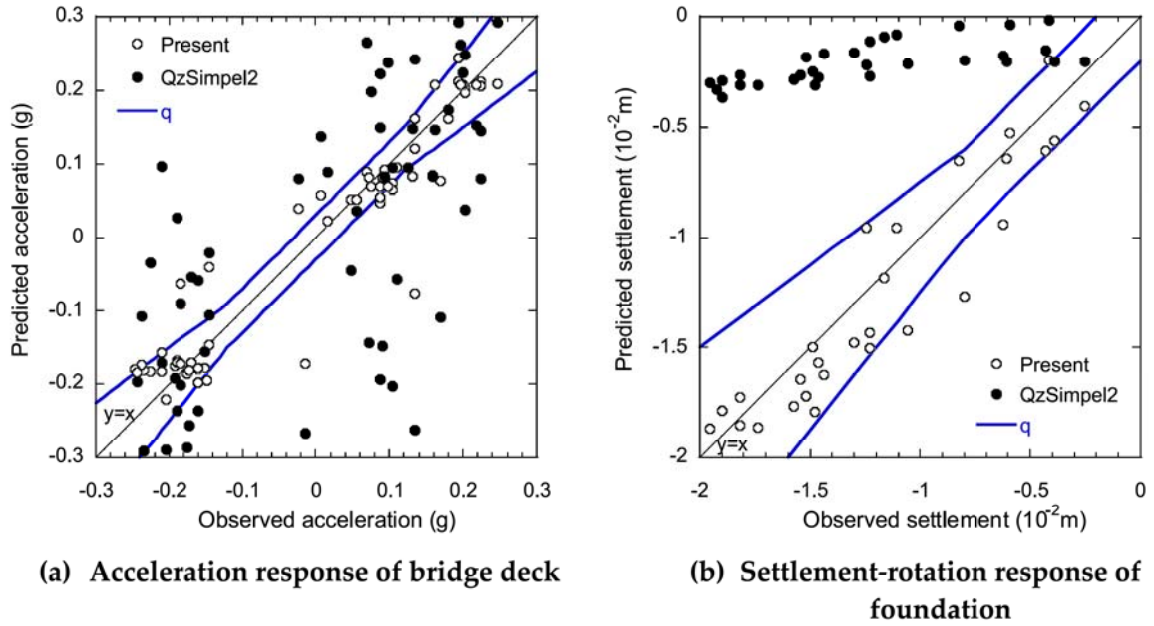
Fig. 5. Scatter plots for comparison between the Winkler model and the experiments for the 0.15 g acceleration amplitude.
