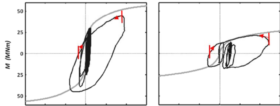
(a) Moment-rotation response: Large foundation (left) and Medium foundation (right)
