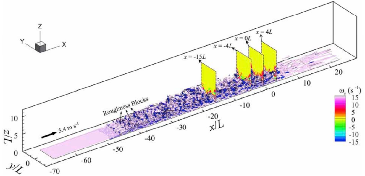
Fig. A-1. Instantaneous flow fields in the absence of hills.
