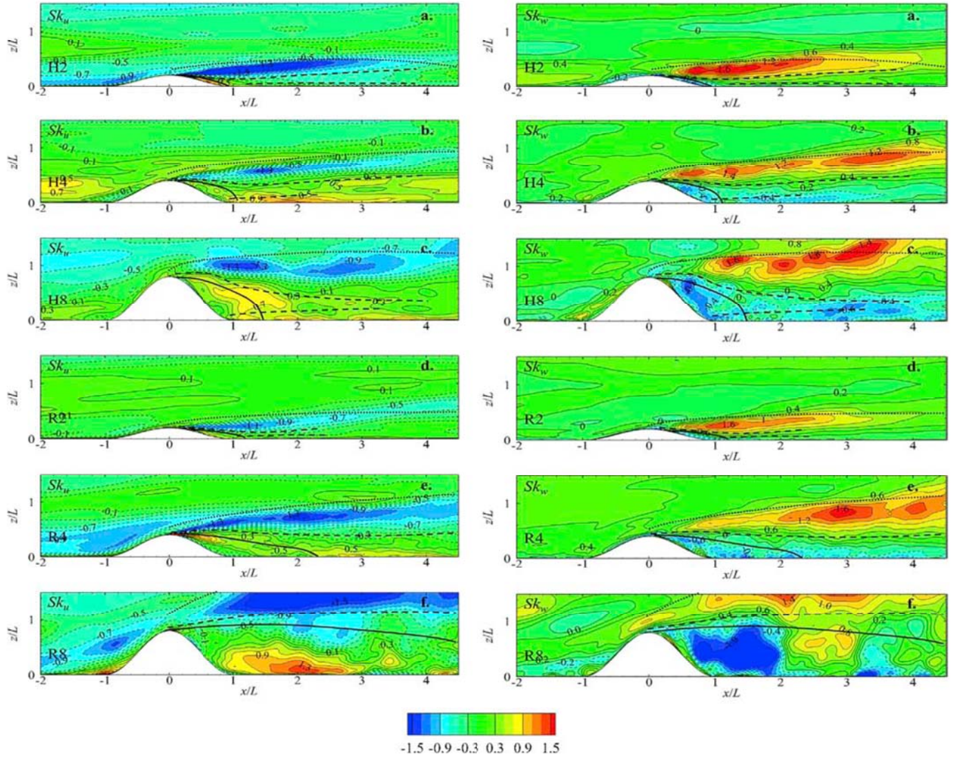
Fig. 7. Distributions of Sk_u for (a) H2, (b) H4, (c) H8, (d) R2, (e) R4, (f) R8, and Sk_w for (g) H2, (h) H4, (i) H8, (j) R2, (k) R4, (l) R8, on the vertical slice of y = 0 . The dotted lines denote the boundary of the wake depth, the dashed lines indicate the locations of peak TKE, and the solid lines show the center of the separation bubble with zero mean streamwise velocities.
