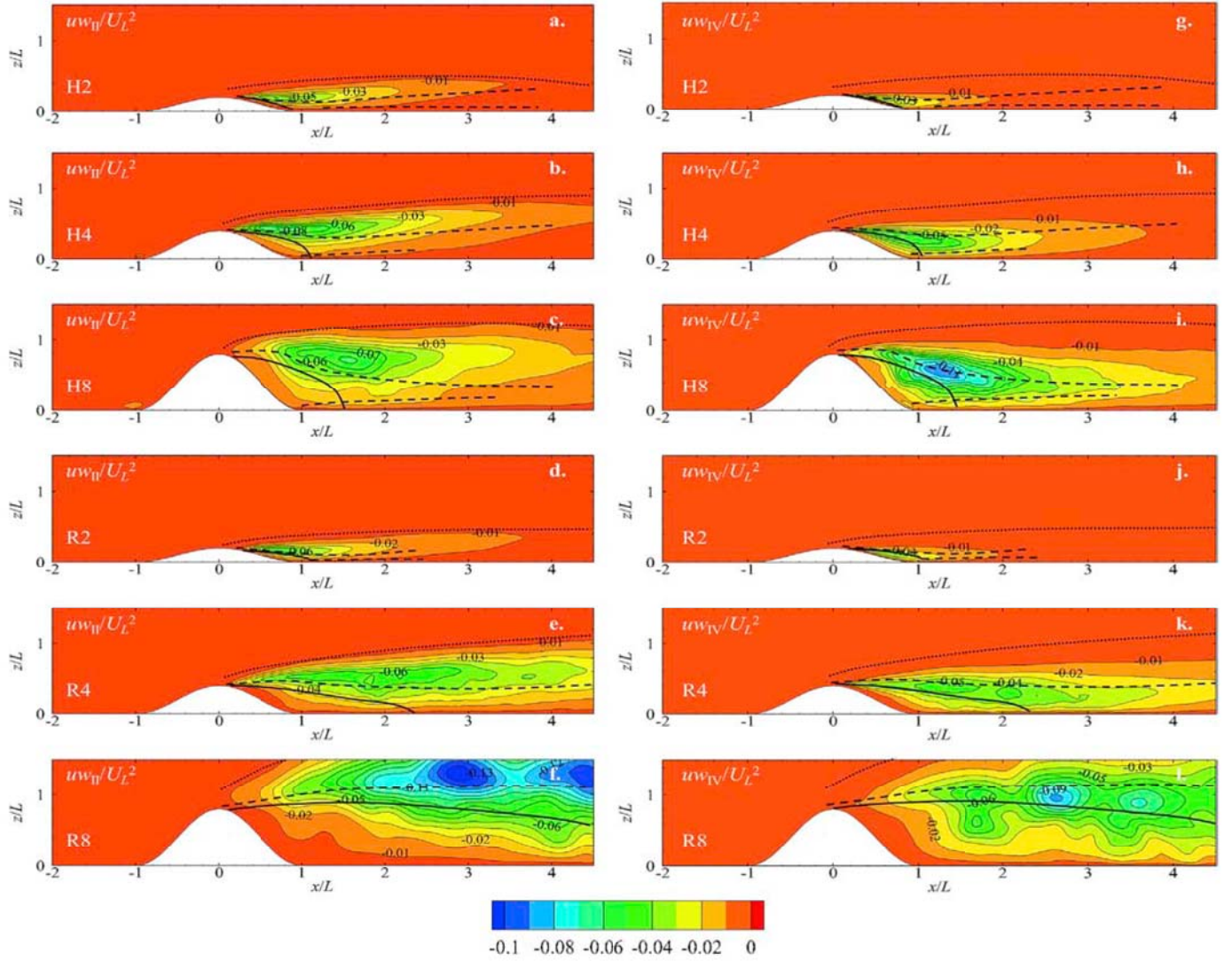
Fig. 5. Distributions of uw_w for (a) H2, (b) H4, (c) H8, (d) R2, (e) R4, (f) R8, and uw_v for (g) H2, (h) H4, (i) H8, (j) R2, (k) R4, (l) R8, on the vertical slice of y = 0 . The dotted lines denote the boundary of the wake depth, the dashed lines indicate the locations of peak TKE, and the solid lines show the center of the separation bubble with zero mean streamwise velocities.
