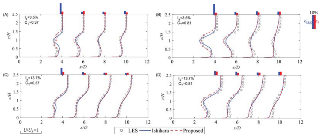
FIGURE 14 Comparisons of the mean streamwise velocities in the vertical direction, when (A) I_a = 3.5\% and C_T = 0.37 , (B) I_a = 3.5\% and C_T = 0.81 , (C) I_a = 13.7\% and C_T = 0.37 , and (D) I_a = 13.7\% and C_T = 0.81 [Colour figure can be viewed at wileyonlinelibrary.com ]
