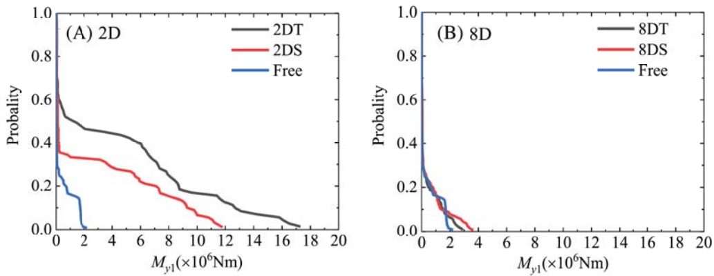
FIGURE 10 Exceedance probability of M_{y1} amplitude at the tower base by rainflow cycle counting when the wind turbine is located at (A) x = 2D and (B) x = 8D [Colour figure can be viewed at wileyonlinelibrary.com ]
