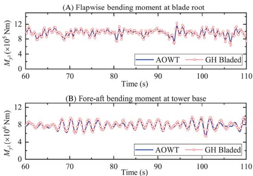
FIGURE 4 Validation of (A) the flapwise bending moments at the blade root and (B) the fore-aft bending moments at the tower base [Colour figure can be viewed at wileyonlinelibrary.com ]
