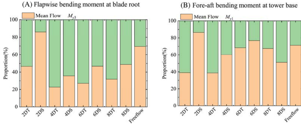
FIGURE 13 Proportion of the fatigue load at (A) the blade root and (B) the tower base, because of the space variation of the mean flow fields [Colour figure can be viewed at wileyonlinelibrary.com ]
