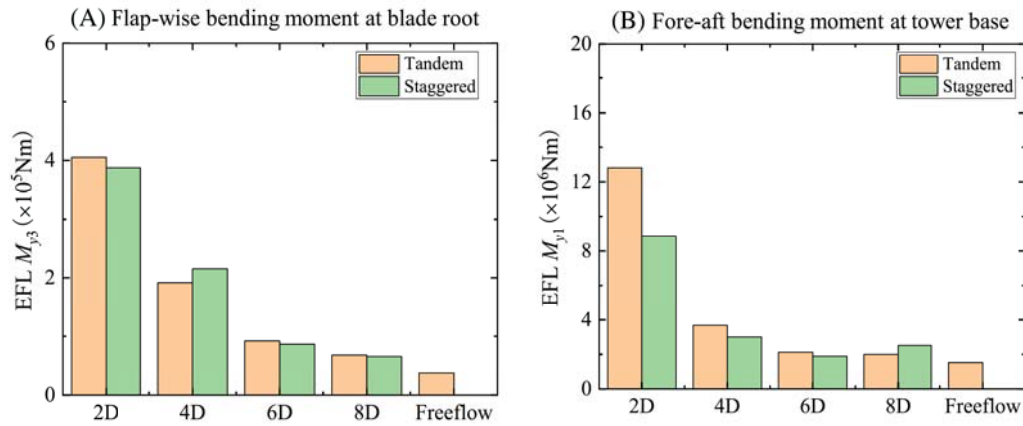
FIGURE 11 Equivalent fatigue loads at (A) the blade root and (B) the tower base, induced by the instantaneous flow fields [Colour figure can be viewed at wileyonlinelibrary.com ]
