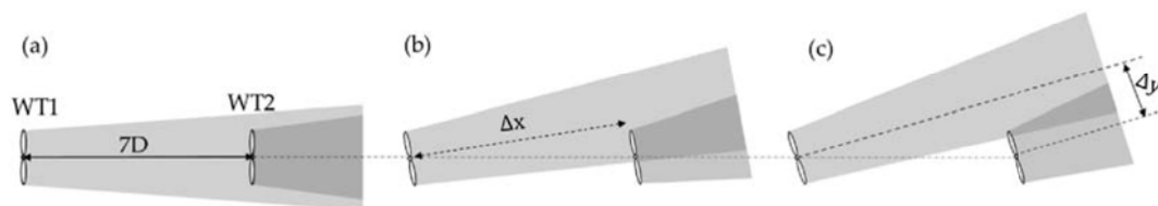
Fig. 2. Wind turbine layouts under different wind directions: (a) In-line with full overlap: wind direction of 0°; (b) Partial offset with partial overlap: wind direction of 5°; (c) Fully offset with partial overlap: wind direction of 10°. D is the diameter of wind turbine rotor. \Delta x and \Delta y are the longitudinal distance and lateral offset, respectively.
