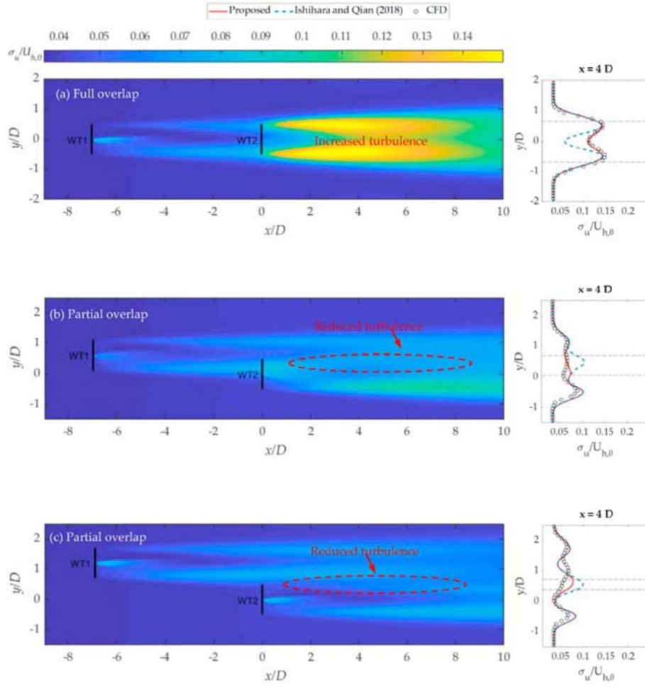
Fig. 7. Contours and profiles of turbulence intensity in the wake of two wind turbines: (a), (b), and (c) are results under wind direction of 0^\circ , 5^\circ and 10^\circ , respectively. The wind turbines are presented by the solid black lines. The dashed lines mark the interaction region in wakes of two turbines. Blue solid lines show the results by directly combining added turbulence intensity individually predicted by Ishihara-Qian model for WT1 and WT2, respectively. Red solid lines present the results predicted by the new multiple wake model. (For interpretation of the references to colour in this figure legend, the reader is referred to the Web version of this article.)
