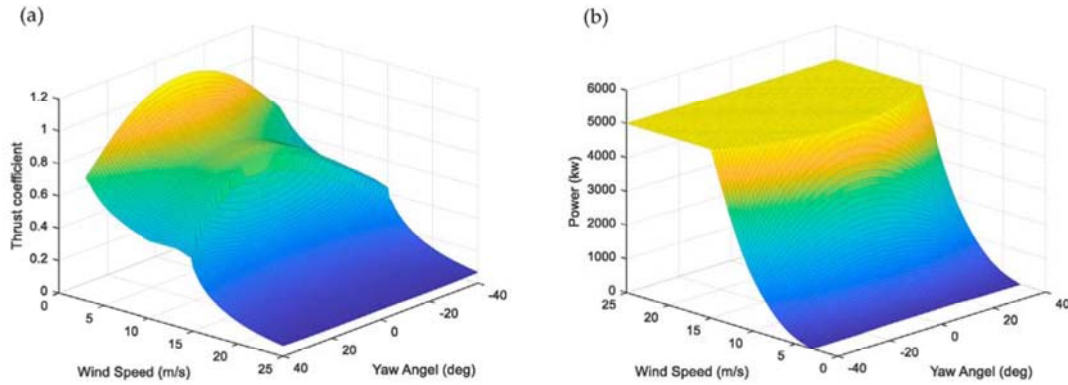
Fig. 4. Thrust coefficient (a) and power curve (b) of the NREL 5-MW reference wind turbine as a function of wind speed U and yaw angle \gamma .
