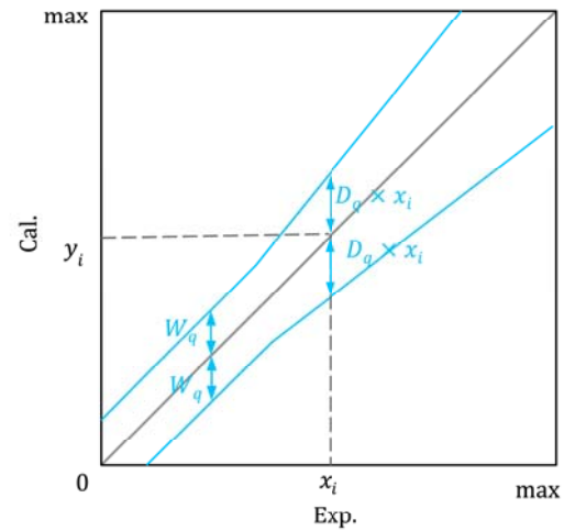
Fig. 1. Schematic of Validation Metrics. The lines in blue mark the boundaries defined by q . (For interpretation of the references to colour in this figure legend, the reader is referred to the Web version of this article.)
