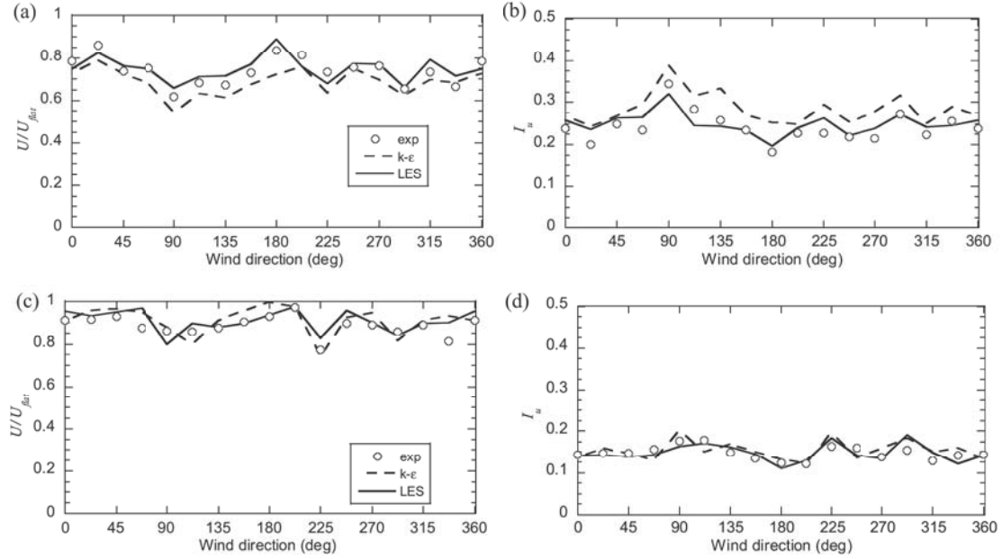
Fig. 24. Comparison between simulation results and experimental data against different wind directions: (a) wind speed ratio and (b) turbulence intensity the height of 13.5 m, (c) wind speed ratio and (d) turbulence intensity the height of 30 m.
