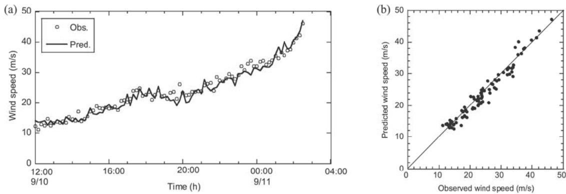
Fig. 28. Comparison of predicted and observed wind speeds at the Miyako Branch: (a) 10-min-average wind speeds and (b) scatter plots.
