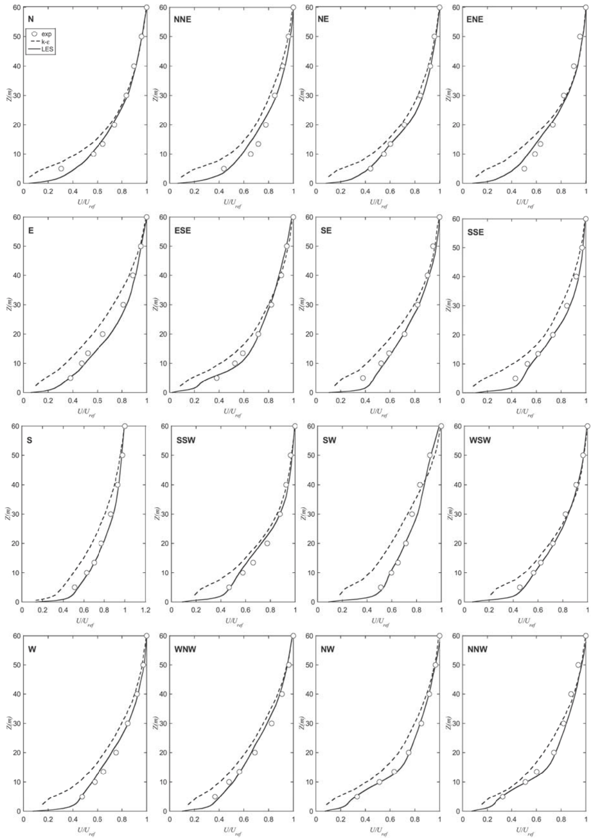
Fig. 22. Vertical profiles of mean wind speed at the target site in each wind direction. Open circles denote experimental data, dash lines are results predicted by the modified k-\epsilon model, and solid lines represent values obtained from LES simulation.
