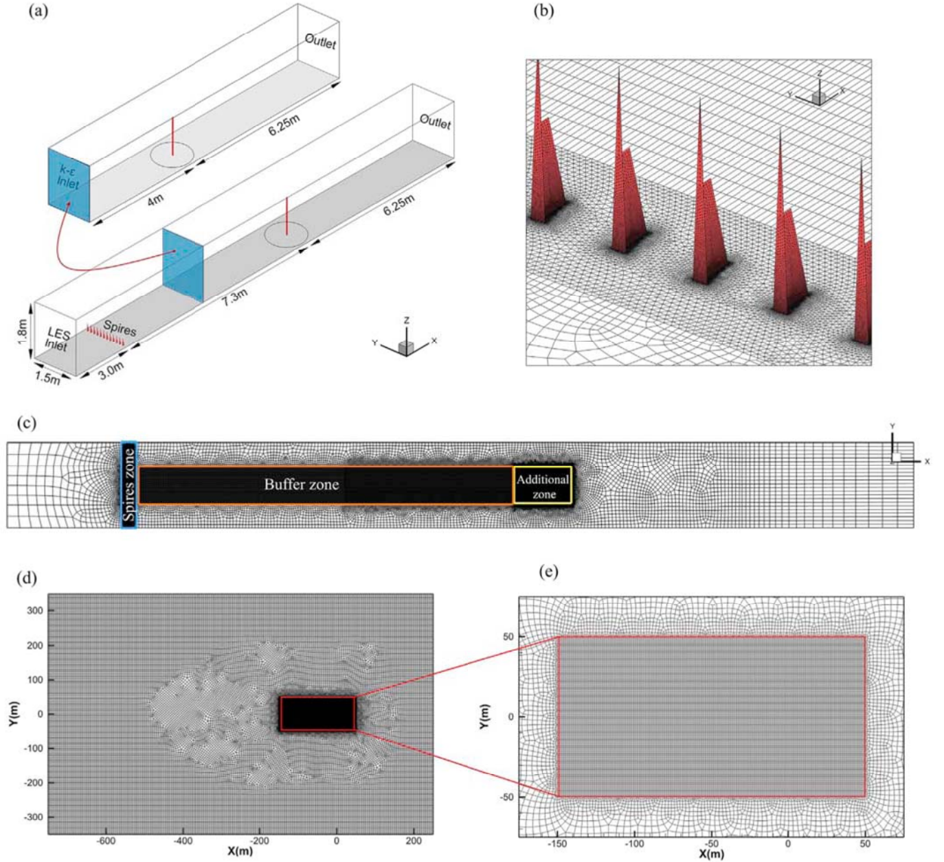
Fig. 17. Configuration of the numerical wind tunnel: (a) bird view of computational domain for LES and modified k-\epsilon model; (b) grid on spires in numerical simulation; (c) grid system, including the buffer zone and the fine grid zone in the urban area; (d) grid arrangement in the additional and target zones around the station at full scale.
