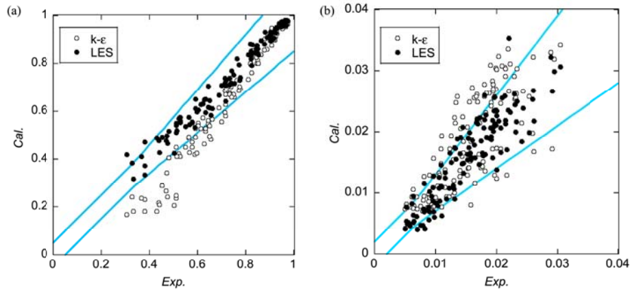
Fig. 25. Scatter plots of numerical simulation results against experimental data for the real urban area: (a) normalized mean wind speed U/U_{ref} , (b) normalized Reynolds stress -\overline{u'w'}/U_{ref}^2 . Blue lines mark the threshold for hit rate q . (For interpretation of the references to colour in this figure legend, the reader is referred to the Web version of this article.)
