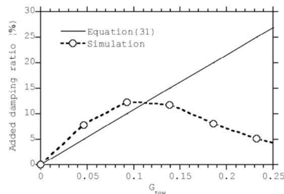
Figure 9. Comparison of theoretical and actual damping ratios of the nacelle acceleration feedback controller for different gain values G_{tow} .
