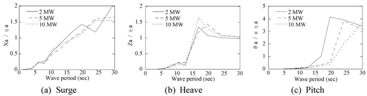
Figure 5. Response Amplitude Operator for each turbine size.
