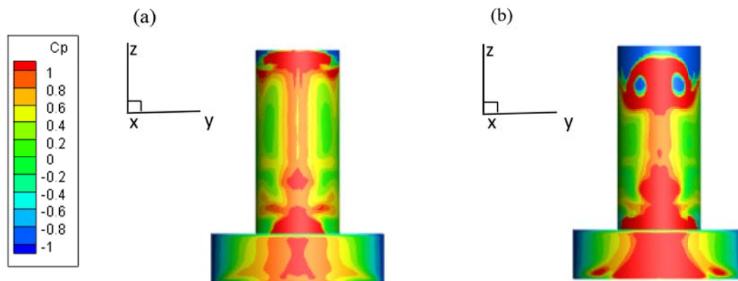
Fig. 13. The nomalized dynamic pressure on the surfaces of HP1 and SC1 at t/T=1 under the free surface in the horizontally forced vibrations with (a) KC=4.62 and (b) KC=9.24
