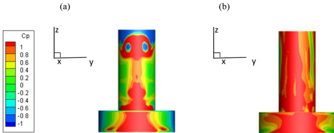
Fig. 17. The normalized dynamic pressure on SC1 and Hp1 under water at t/T=1 (a) with and (b) without the effect of free surface in the horizontally forced vibration for KC=9.24 and T=1.8s
