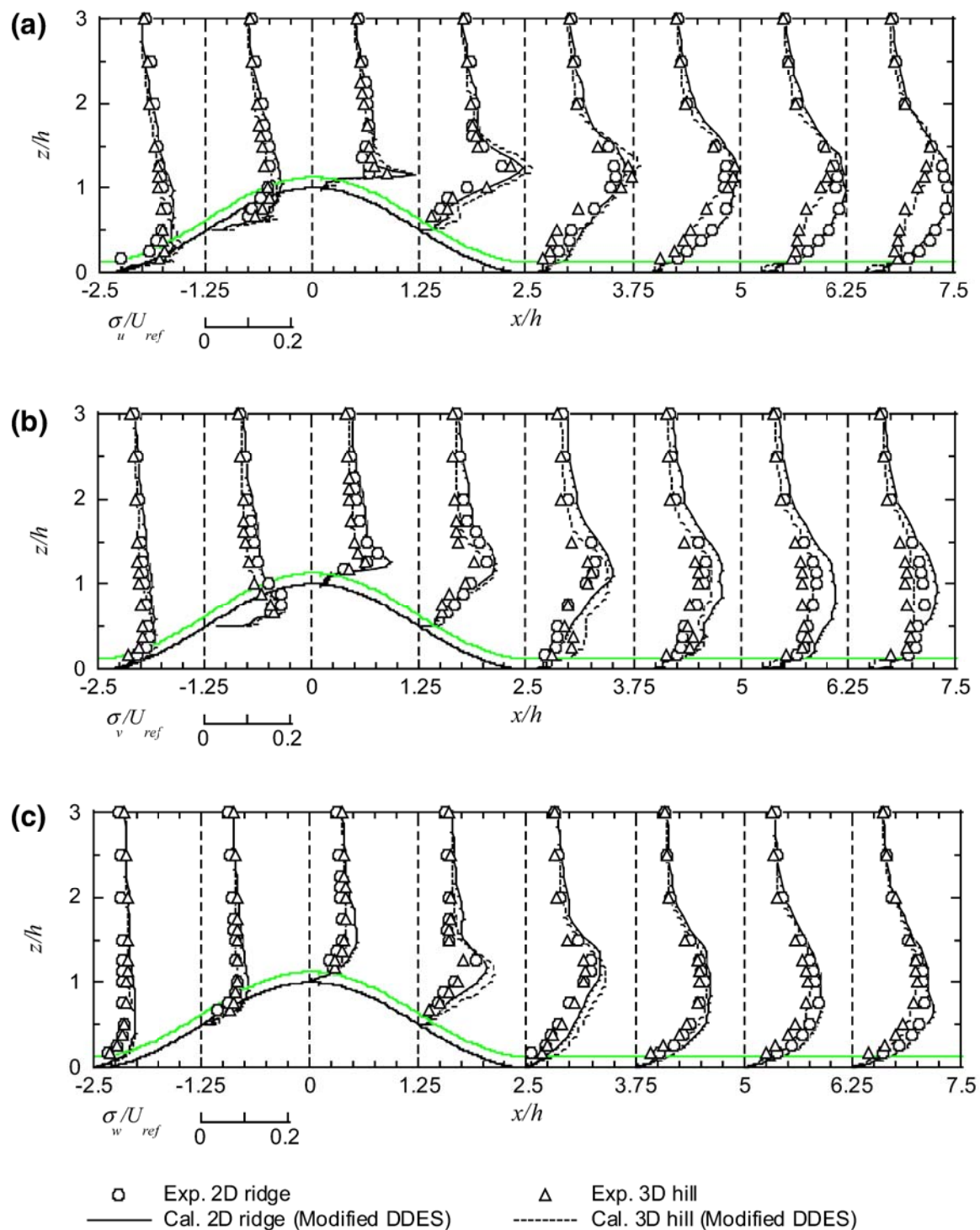
Fig. 7 Predicted and measured a longitudinal, b lateral and c vertical normal stress components over the two-dimensional rough ridge and the three-dimensional rough hill in the central plane of terrain
