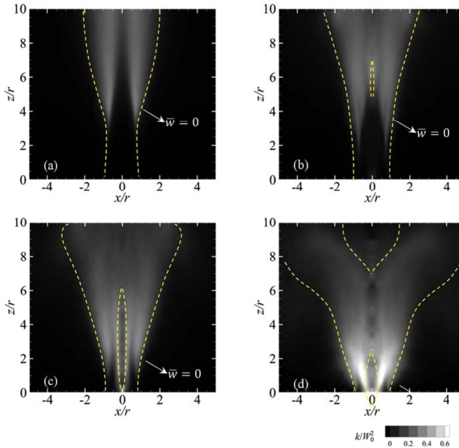
Fig. 11. TKE (averaged in \theta direction) distribution on the central slice with horizontal and vertical axis normalized by the radius of chamber outlet r . Yellow dashed lines are the contour lines of \bar{w} = 0 . (a) Case1, (b) Case2, (c) Case3 and (d) Case4. (For interpretation of the references to color in this figure legend, the reader is referred to the Web version of this article.)
