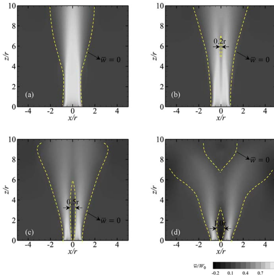
Fig. 8. Mean axial velocity (averaged in time and \theta direction) distribution on the central slice with horizontal and vertical axis normalized by the radius of chamber outlet r and values of the axial velocity by the averaged axial velocity at the chamber outlet W_0 . Yellow dashed lines are the contour lines of \bar{w} = 0 . (a) Case1, (b) Case2, (c) Case3 and (d) Case4. (For interpretation of the references to color in this figure legend, the reader is referred to the Web version of this article.)
