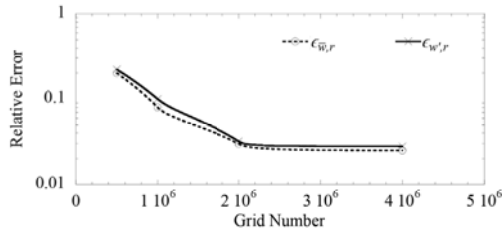
Fig. 4. Relative errors of mean axial velocity \varepsilon_{w,r} , and rms of axial velocity, \varepsilon_{w',r} , versus grid number with horizontal axis increasing linearly and vertical axis logarithmically.
