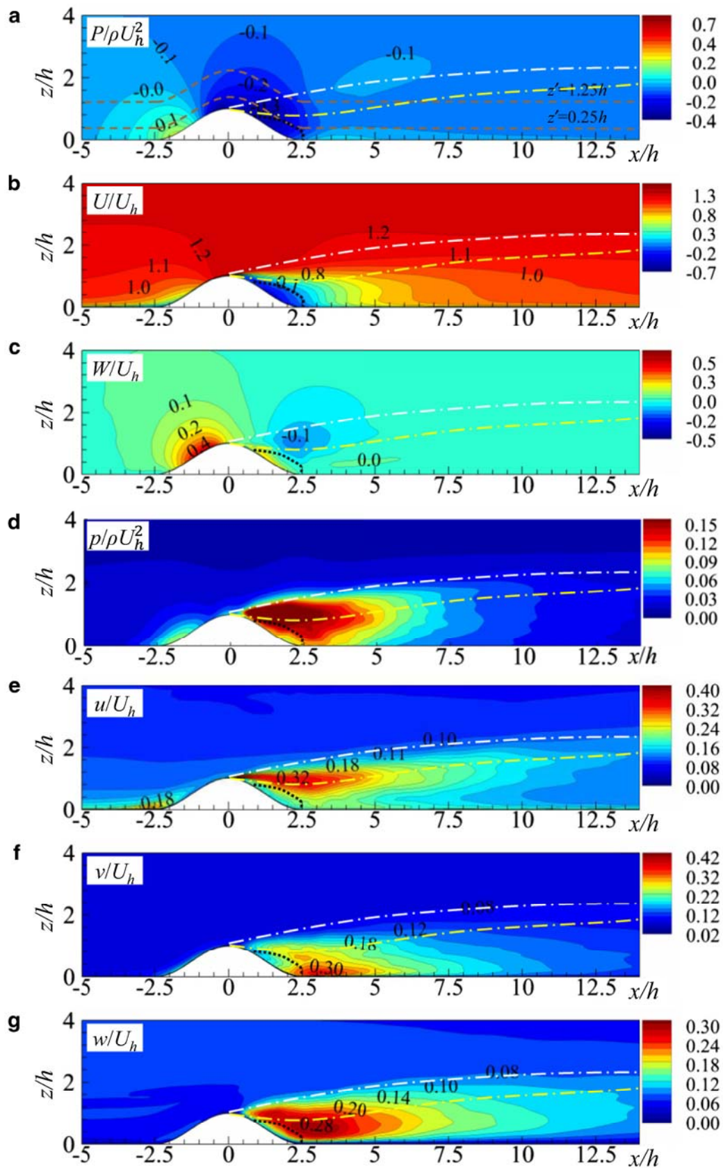
Fig. 5 Vertical cross-sections through y = 0 of the mean a pressure, and b streamwise and c vertical velocity components, and the r.m.s. of d pressure, and e streamwise, f spanwise, and g vertical velocity components. The brown, thin dashed lines in a are the locations of the flow fields discussed in Sects. 3.2 and 3.3. The white and yellow dash-dot lines denote the boundaries of the wake depth and shear layer, respectively. The thick, black dashed lines show the boundary of the separation bubble with zero mean streamwise velocity. The x - and z -axes are normalized by the height h
