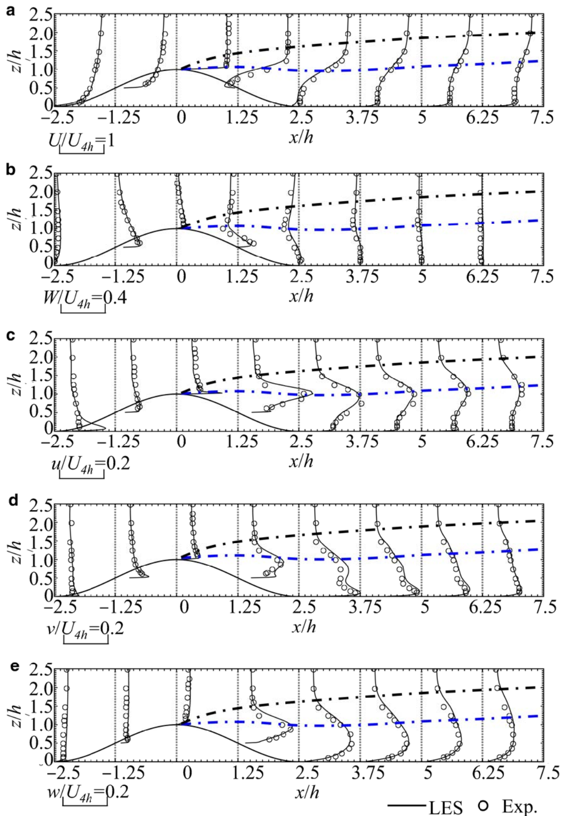
Fig. 3 Profiles of the mean and fluctuating velocity components on the vertical cross-section at y = 0 : mean of the a streamwise, and b vertical velocity components, and r.m.s. of the c streamwise, d spanwise, and e vertical velocity components. The black and blue dash-dot lines are the wake depth and the shear layer, respectively. The x - and z -axes are normalized by the height h . The red points with z' = 1.25h denote the reference points for the calculations of the space correlations in Sect. 3. The velocities U_i and u_i are normalized by the wind speed U_{4h}
