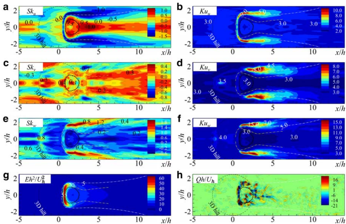
Fig. 11 Contours of skewness of a streamwise Sk_u , c spanwise Sk_v , and e vertical Sk_w velocity components, and kurtosis of b streamwise Ku_u , d spanwise Ku_v , and f vertical Ku_w , velocity components, the g mean enstrophy, and h instantaneous Q-criterion on the plane z' = 0.25h . The white and yellow dash-dot lines denote the boundaries of the wake depth and the shear layer, respectively. The thin, black dashed circle indicate the 3D hill. The thick, black dashed lines show the boundary of the separation bubble with zero mean streamwise velocities. The x - and y -axes are normalized by the height h
