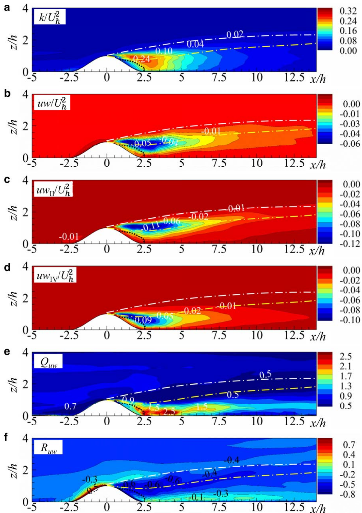
Fig. 6 Distributions of the normalized a TKE, b vertical momentum flux uw , c vertical momentum flux in the second quadrant, uw_{II} , d vertical momentum flux in the fourth quadrant, uw_{IV} , e ratio between the vertical momentum flux in the fourth and second quadrants, Q_{uw} , and f the correlation coefficient between streamwise and vertical velocity components R_{uw} through the cross-section at y = 0 . The white and yellow dash-dot lines denote the boundaries of the wake depth and the shear layer, respectively. The black, dashed lines show the boundary of the separation bubble with zero mean streamwise velocity. The x - and z -axes are normalized by the height h
