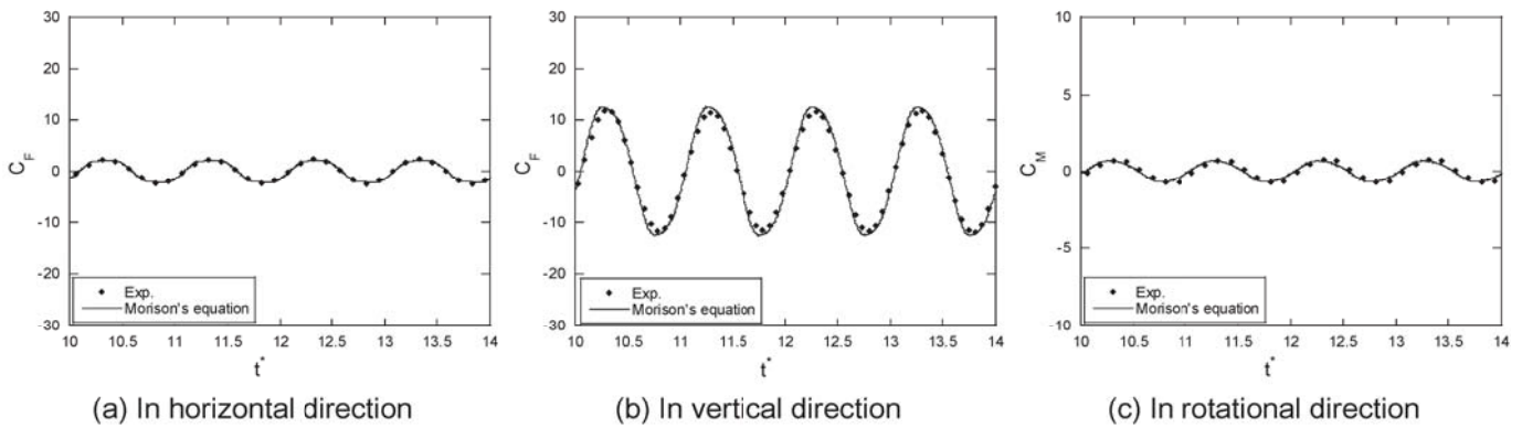
Fig. 9. Measured and predicted time history of force coefficient by Morison's equation in the forced oscillation.
