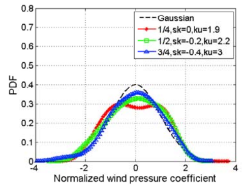
(b) Curved roof ( f_m=10\text{Hz} )
