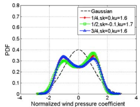
(c) Curved roof ( f_m=30\text{Hz} )
