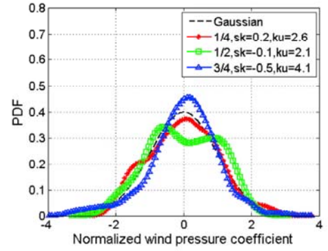
(a) Curved roof ( f_m=0\text{Hz} )
