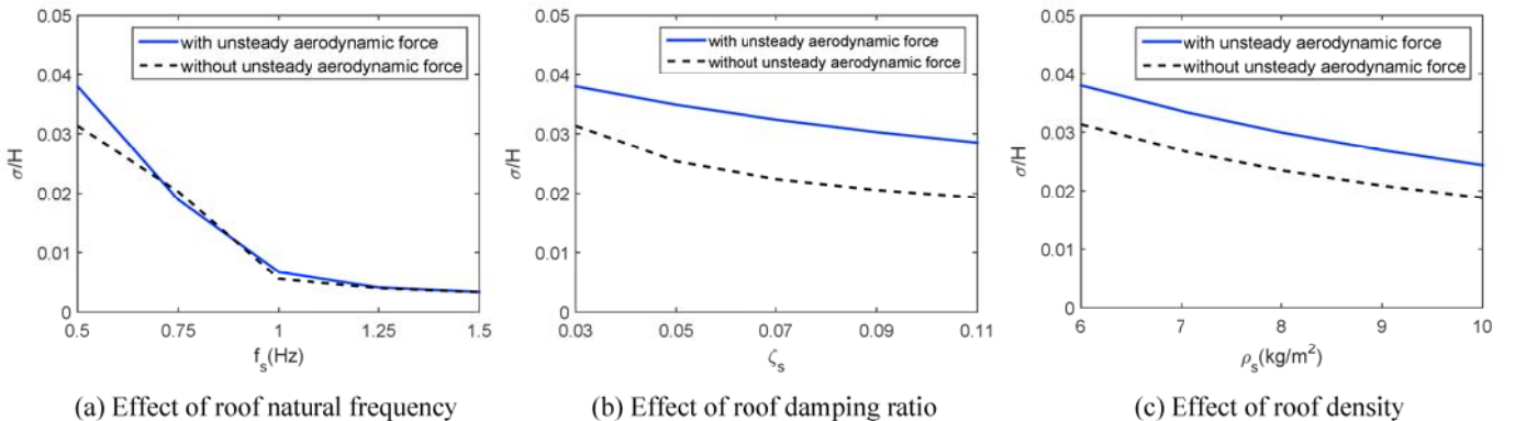
Fig. 23. Variations of standard deviation of generalized displacement with structural parameters.
