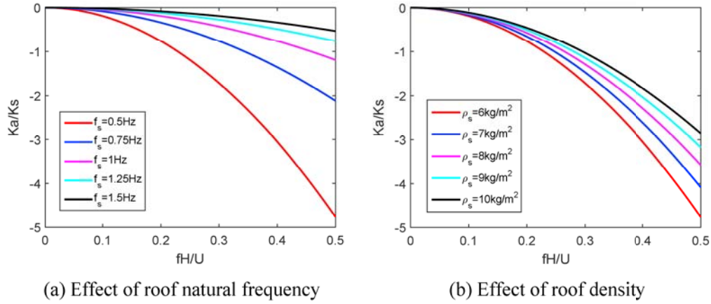
Fig. 19. Aerodynamic stiffness ratios.
