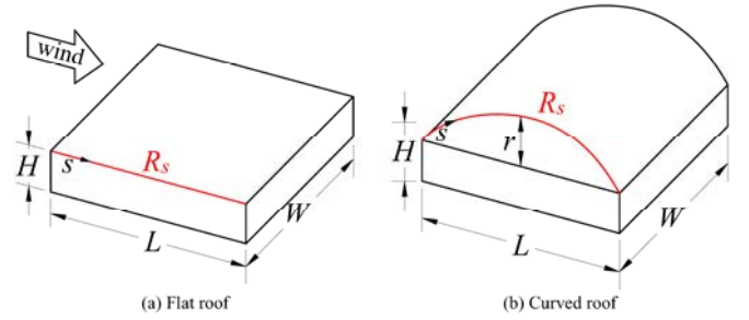
Fig. 1. Geometry of roof model.
