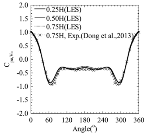
Fig. 6. Mean external pressure coefficient distributions on the cooling tower exposed to the straight-line wind.
