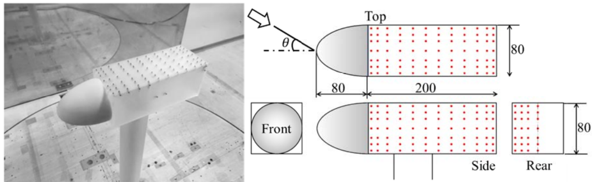
Figure 3. Design and dimensions of the nacelle model. Pressure orifices are distributed on the top, one of the sides and rear surfaces.
