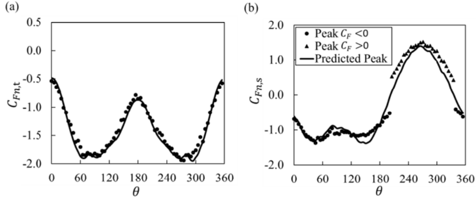
Figure 9. Comparison between predicted and measured forces coefficients on the (a) top and (b) side surfaces of the nacelle for inflow turbulence intensity 13.2%.
