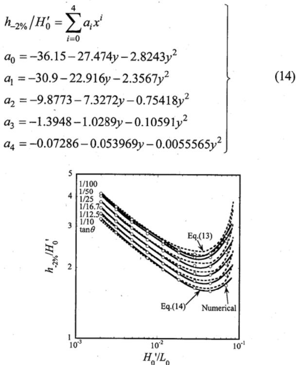
Fig.8 Incipient breaking depth.
