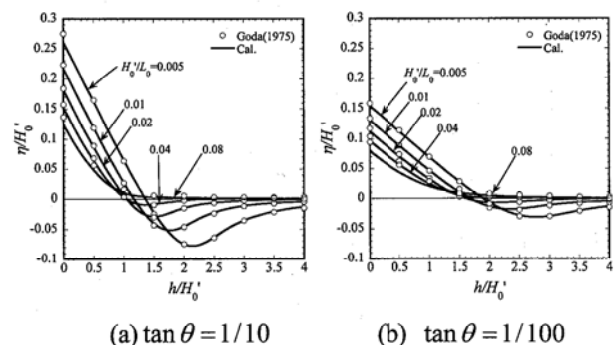
Fig.3 Present numerical results and Goda's water depths.
