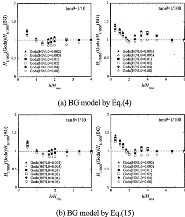
Fig.12 Comparison of H_{1/1000} by Battjes & Groenendijk model and Goda model.
