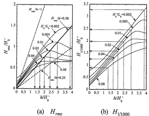
Fig.10 Solution procedure of obtaining H_{1/1000} from H_{rms}/h ( H_{rms}/h = 0.38 , \tan \theta = 1/100 ).
