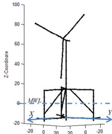
(b) FEM model
