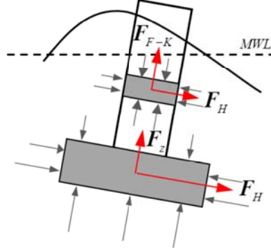
Figure 3: Illustration of hydrodynamic force acting on segment of cylinder and heave plate
