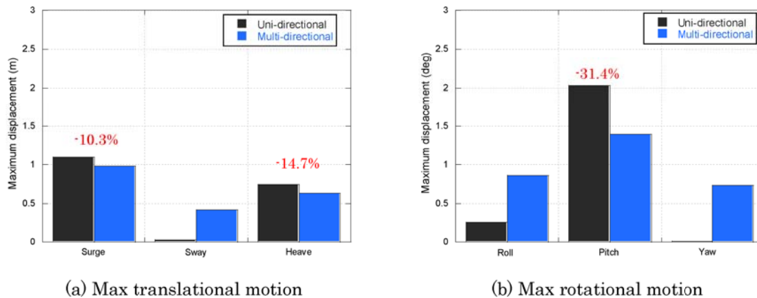
Figure 8: Maximum of (a) translational displacement and (b) rotational motion in unidirectional and multidirectional sea state
