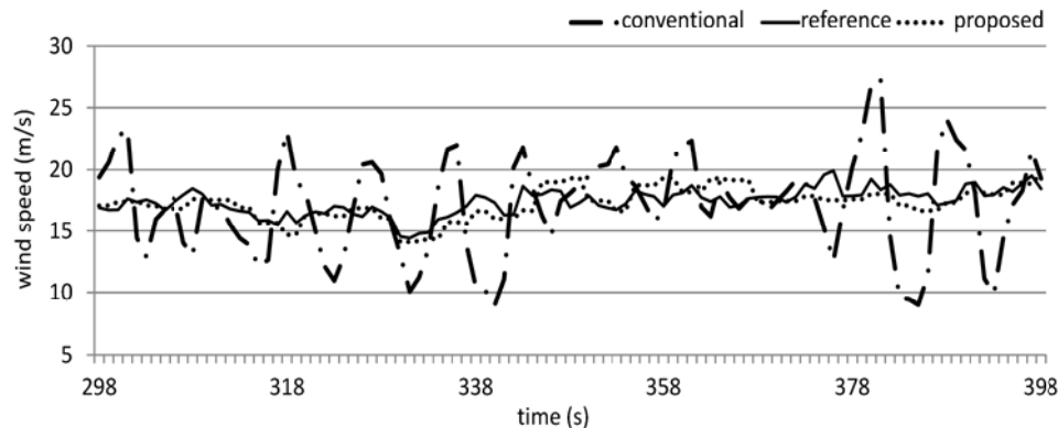
Figure 7 time history of instantaneous wind speed
