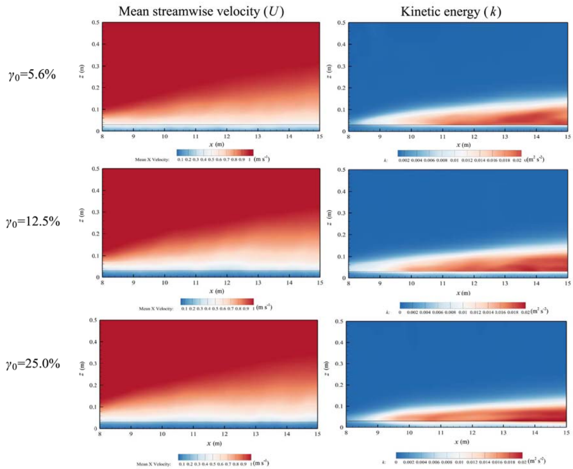
Fig. 5. Contour of mean streamwise velocity and kinetic energy of the flow over roughness blocks with density of 5.6%, 12.5% and 25% computed in fine grid system.
