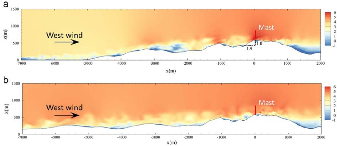
Fig. 20. Instantaneous flow fields visualized by streamwise velocity over the terrain with R equals to (a) 4 km; (b) 8 km; when the wind is from west.
