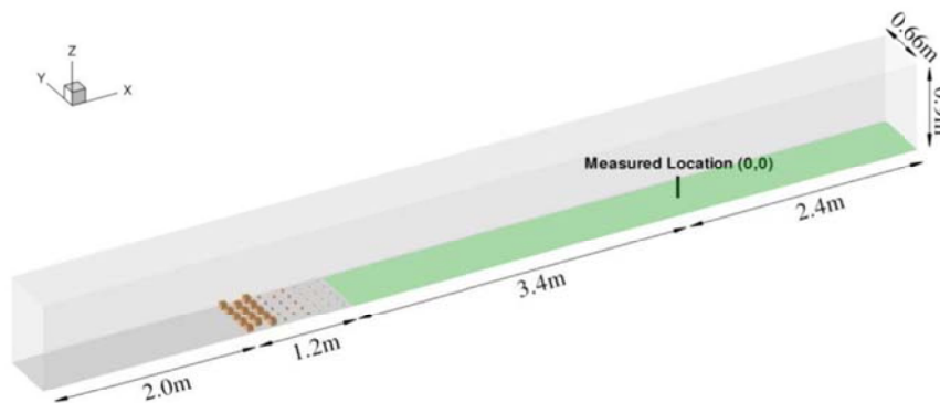
Fig. 7. Configuration of numerical model simulating flat terrain covered by vegetation canopy.
