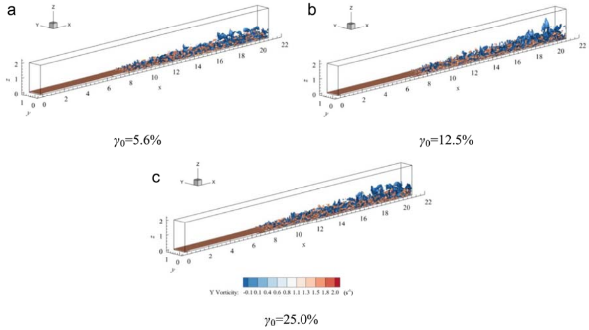
Fig. 4. Vorticity isosurfaces of the turbulent flow fields computed in fine grid system over roughness blocks with density of (a) 5.6%, (b) 12.5% and (c) 25%. Unit: meter.
