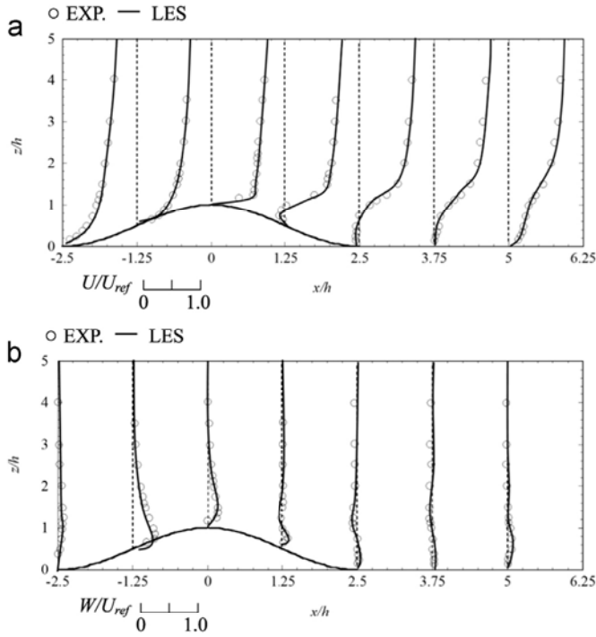
Fig. 14. Profiles of the normalized mean velocities of the flow over 3-D hill covered by vegetation canopy, (a) streamwise component and (b) vertical component on the vertical slice crossing y=0 .
