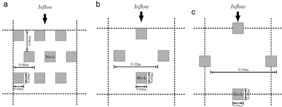
Fig. 1. Arrangement of roughness blocks with density of (a) 25.0%, (b) 12.5% and (c) 5.2%.
