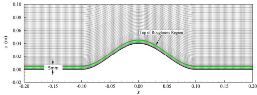
Fig. 12. Distributions of the mesh on the vertical slice crossing the center of the 3-D hill covered by vegetation canopy.
