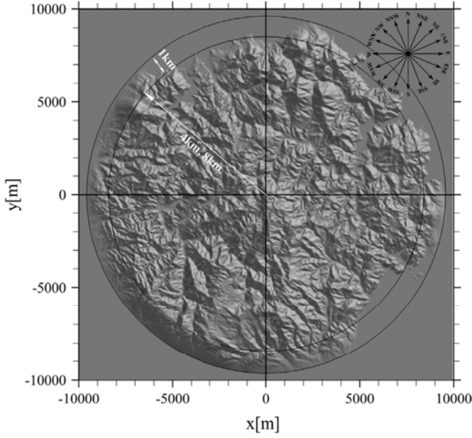
Fig. 16. Topography map of the terrain near Taikoyama hill, Kyoto, Japan.
