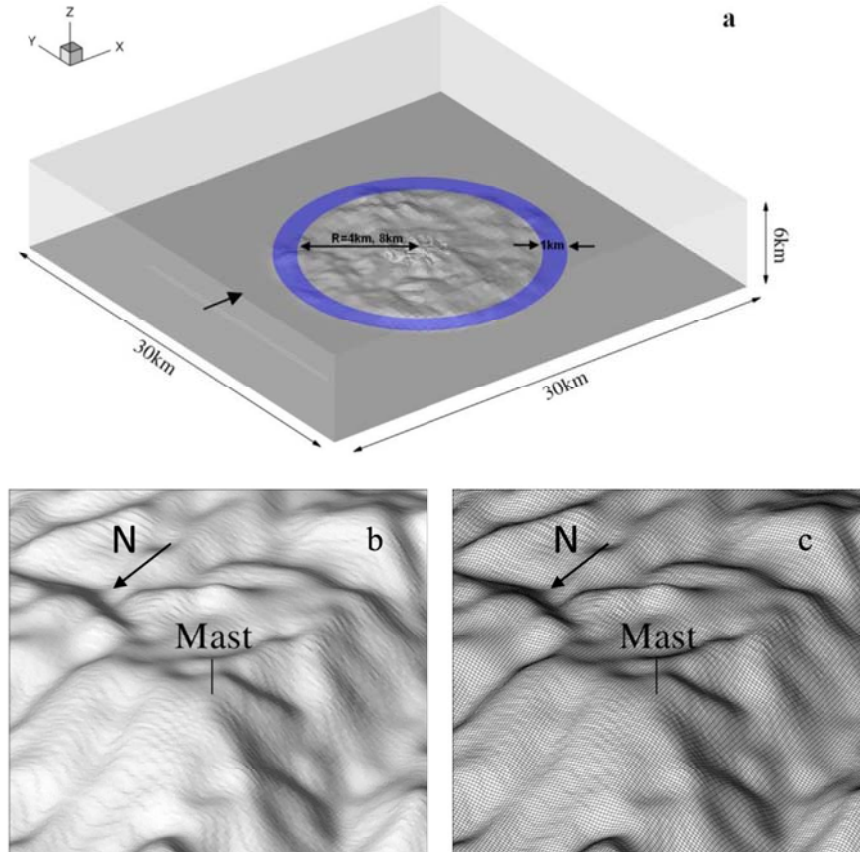
Fig. 17. Configuration of numerical model simulating Taikoyama hill, (a) global view of model; (b) terrain near the Mast; and (c) mesh near the Mast.
