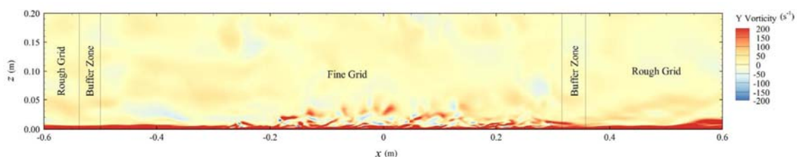
Fig. 9. Turbulence features of the flow over flat terrain covered by vegetation on the vertical slice crossing y=0 .
