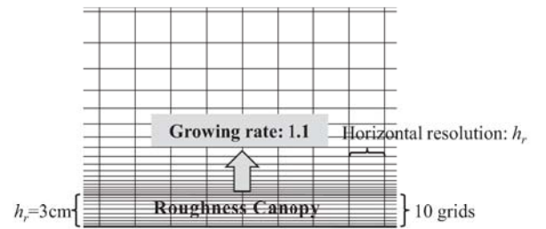
Fig. 3. Vertical grid distribution of the numerical wind tunnel simulating the roughness blocks canopy (fine grid case).
