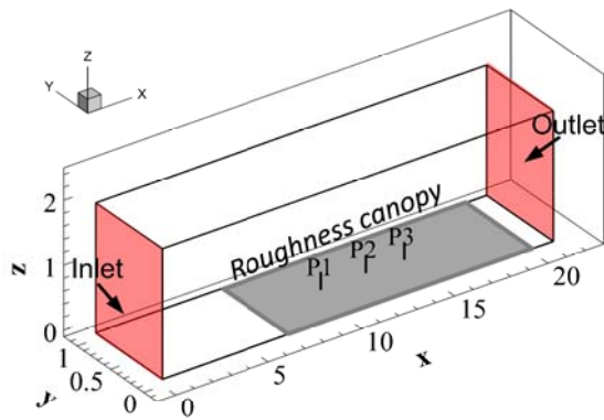
Fig. 2. Configuration of the numerical wind tunnel simulating the canopy of roughness blocks. Unit: meter.
