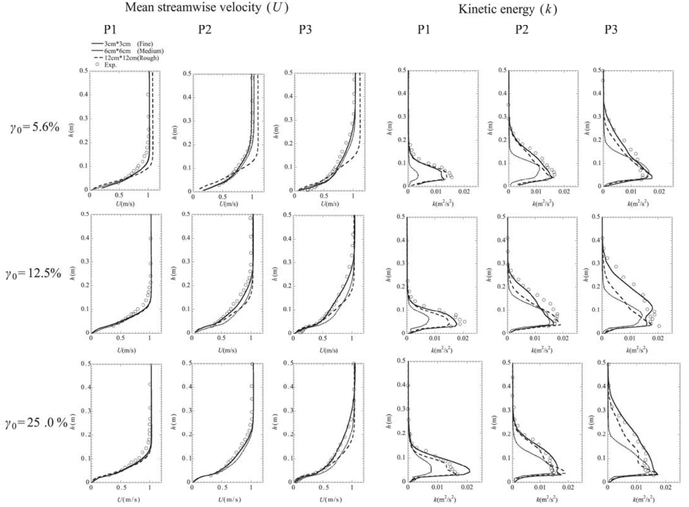
Fig. 6. Comparison of the profiles of mean streamwise velocity and kinetic energy of the flow roughness blocks with density of 5.6%, 12.5% and 25% from models with different horizontal resolutions and the experiments.
