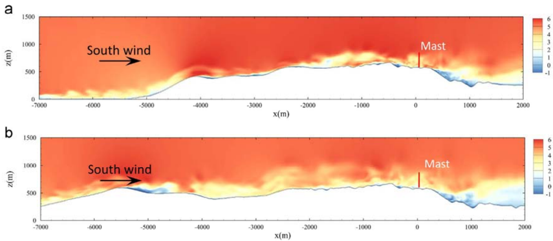
Fig. 21. Instantaneous flow fields visualized by streamwise velocity over the terrain with R equals to (a) 4 km; (b) 8 km; when the wind is from south.
