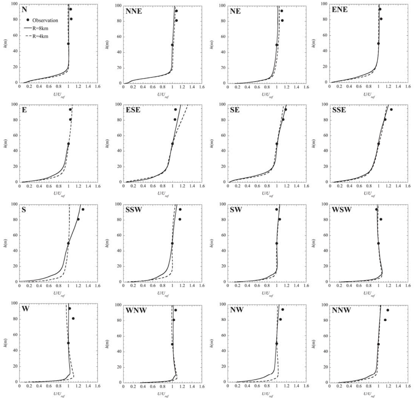
Fig. 18. Profiles of the normalized mean streamwise velocity under sixteen wind directions for the case of Taikoyama hill.
