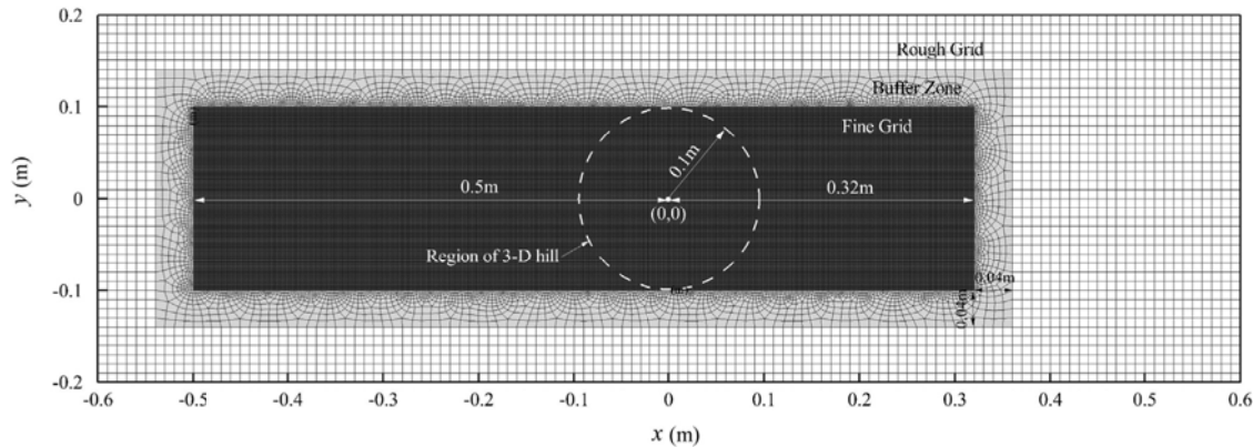
Fig. 8. Sketch map of the locations of the rough grid, buffer zone, and fine grid of the nested grid simulating flat terrain covered by vegetation canopy. White dashed line presents the region covered by a 3-D hill.
