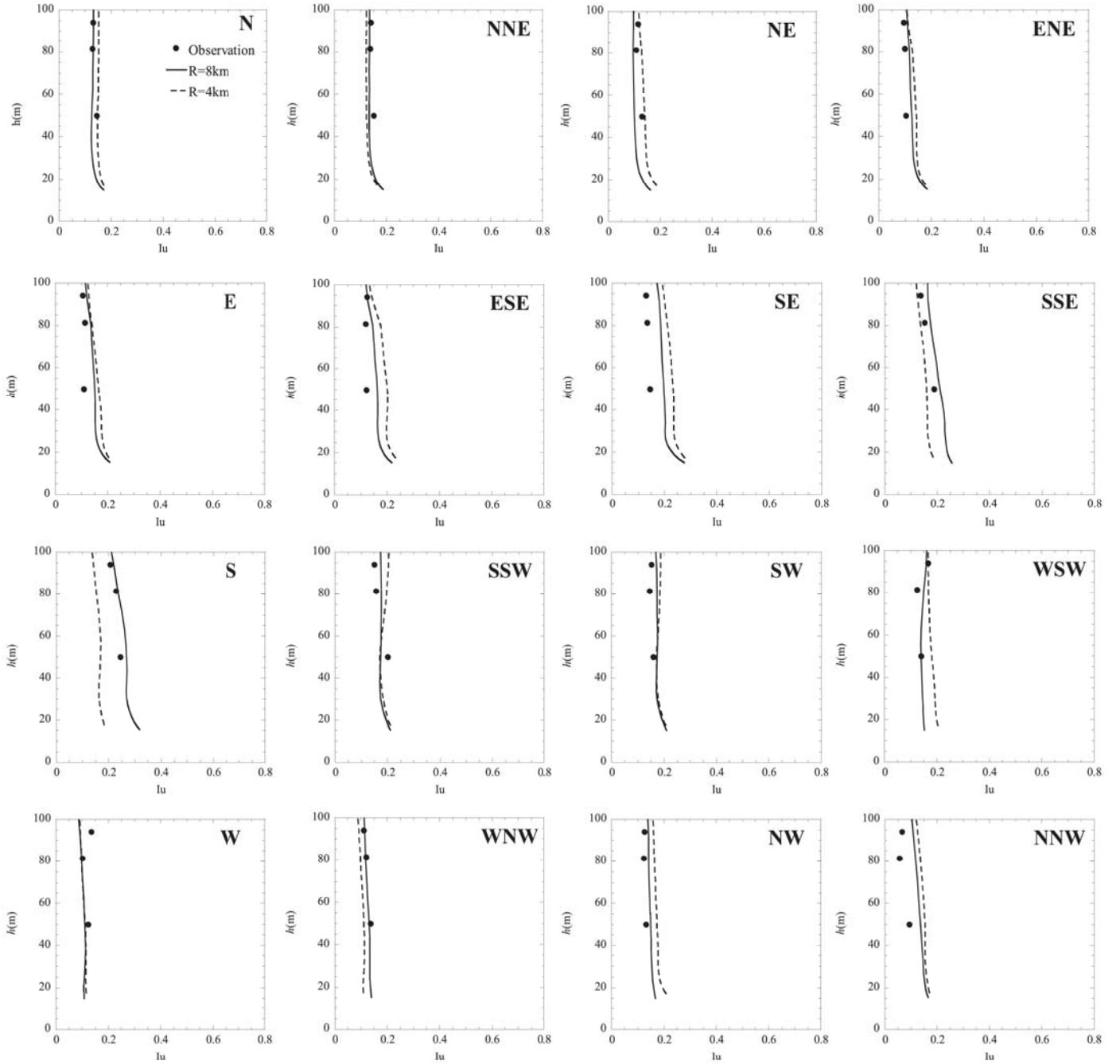
Fig. 19. Profiles of the turbulence intensity at sixteen wind directions for the case of Taikoyama hill.
