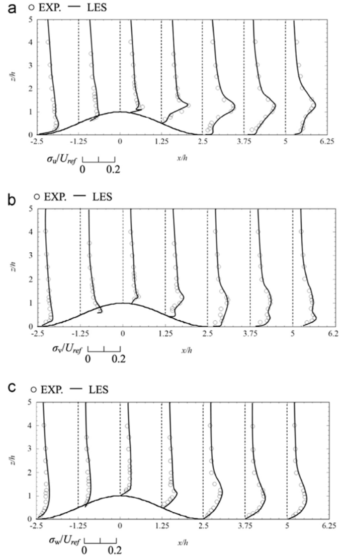
Fig. 15. Profiles of the normalized turbulence fluctuations of the flow over a 3-D hill covered by vegetation canopy, (a) streamwise component, (b) spanwise component and (c) vertical component on the vertical slice crossing y=0 .
