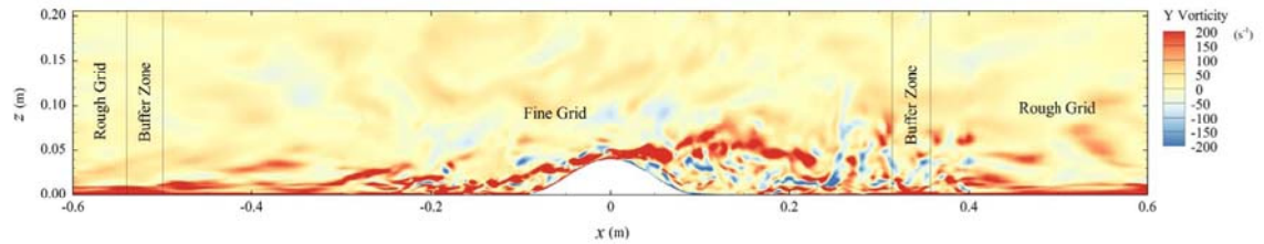
Fig. 13. Turbulence features of the flow over a 3-D hill covered by vegetation on the vertical slice crossing y=0 .
