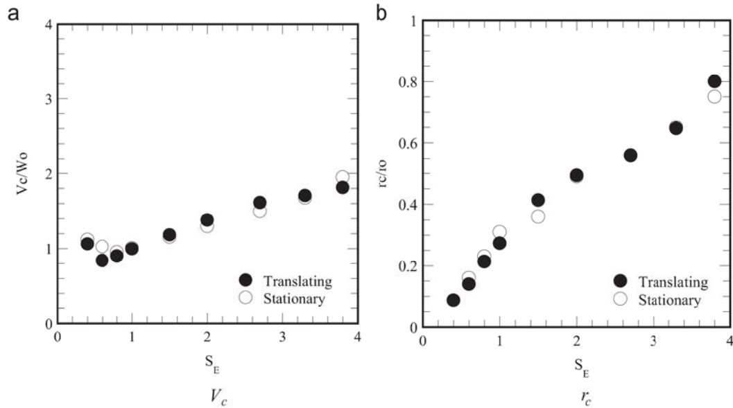
Fig. 21. Comparison of (a) V_c and (b) r_c between translating and stationary tornadoes.
