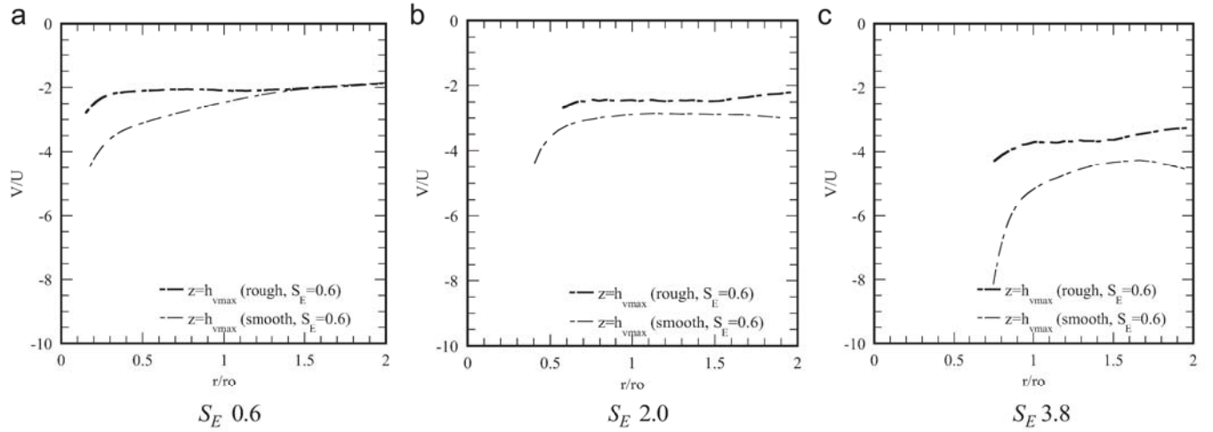
Fig. 38. Comparison of radial profiles of V/U at z = h_{v \max} between tornados over rough and smooth grounds.
