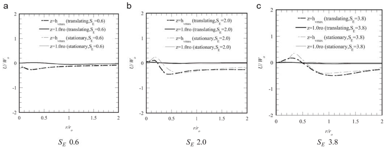
Fig. 22. Comparison of radial profiles of the radial velocity between translating and stationary tornadoes.
