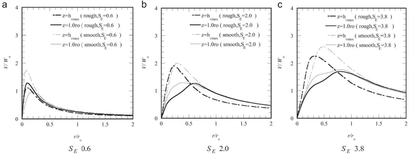
Fig. 35. Comparison of radial profiles of the tangential velocity between tornado over rough ground and that over smooth ground.
