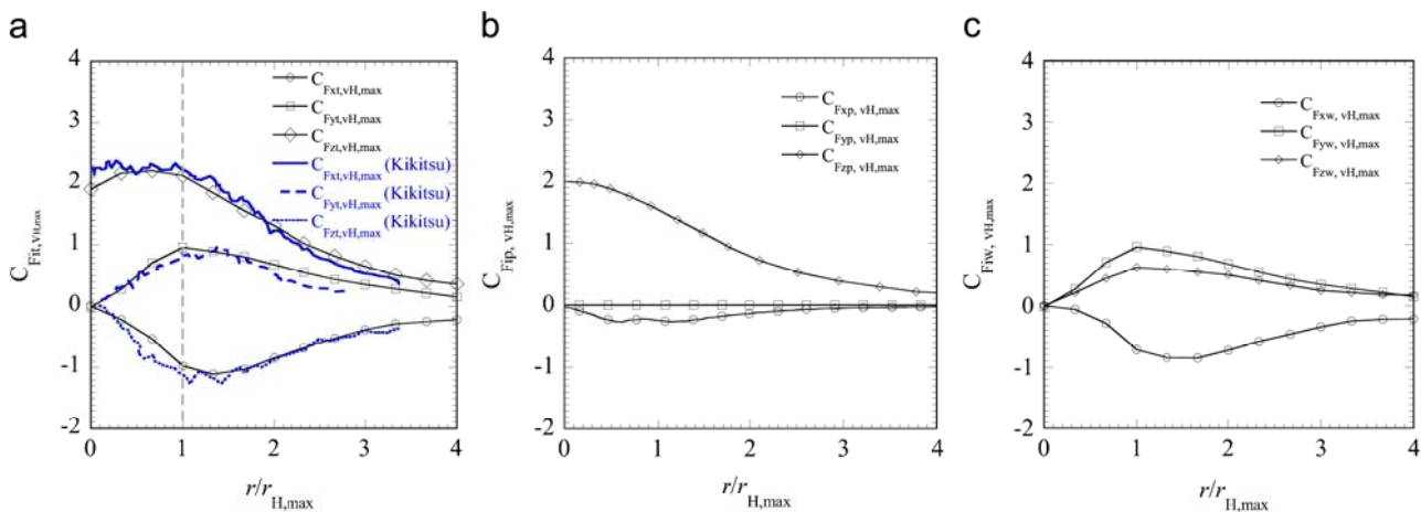
Fig. 6. Radial distribution of the force coefficients, (a) C_{Fit,vH,max} , (b) C_{Fip,vH,max} , and (c) C_{Fiw,vH,max} , from numerical tornado simulator.
