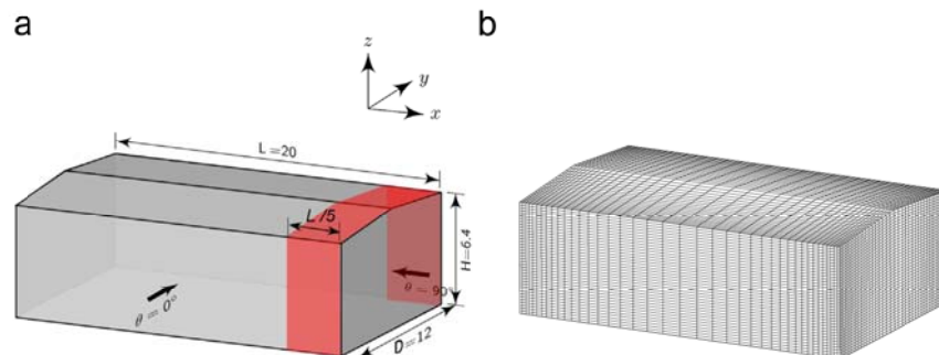
Fig. 1. Building model, (a) geometry and (b) grid (mm) (For interpretation of the references to color in this figure legend, the reader is referred to the web version of this article).
