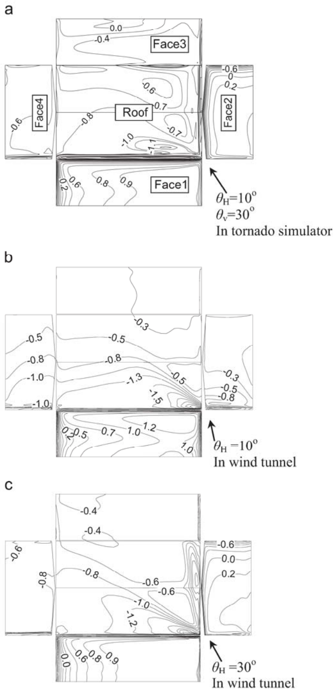
Fig. 16. Mean pressure contour on building model when located at, (a) the outer boundary of tornado core in tornado simulator with \theta_H=10^\circ and \theta_v=30^\circ , (b) in wind tunnel with angle of attack \theta being 10^\circ and (c) angle of attack \theta being 30^\circ .
