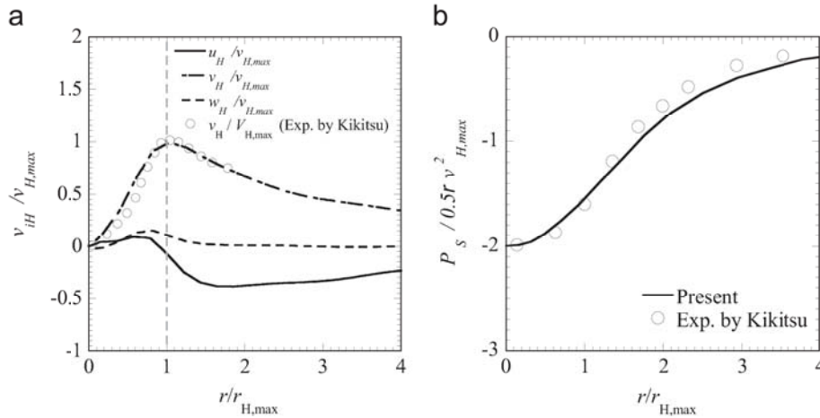
Fig. 5. Flow fields in the simulated tornado with absence of building. (a) Profiles of velocity components at mean eave height, and (b) pressure coefficient on the ground of simulator.
