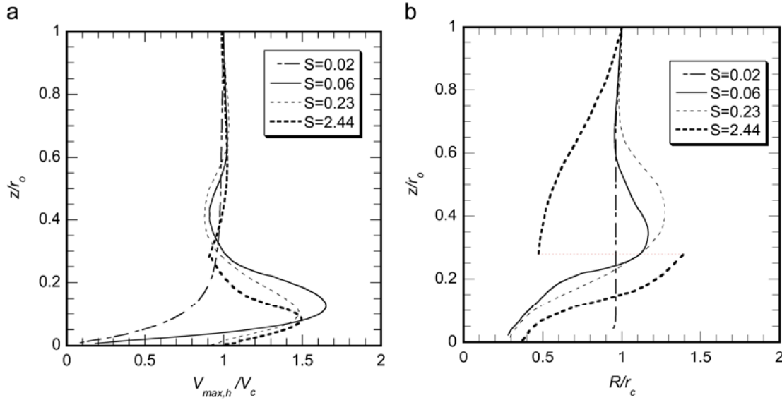
Fig. 9. Vertical distribution of (a) the maximum tangential velocity and (b) the core radius with respect to height.
