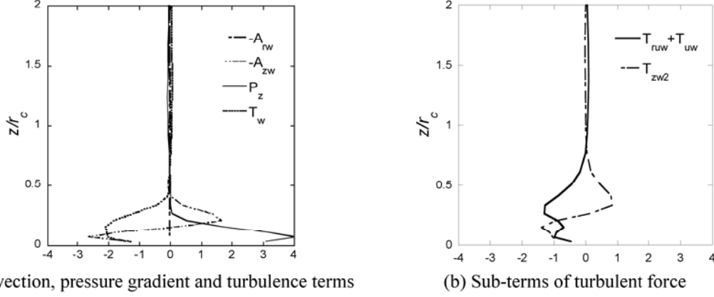
Fig. 10 Vertical distribution of normalized vertical force terms at r = 0r_c , with (a) representing advection, pressure gradient and turbulence terms, and (b), the sub-terms of turbulent force
