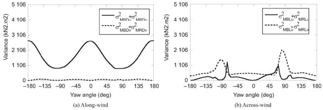
Figure 11. Comparison of standard deviation from u and v (400kW, T_{uh} = 0.158 )
