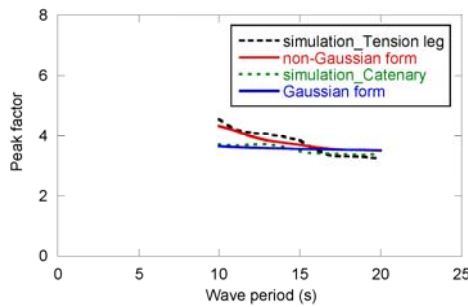
Fig. 11 Comparison of peak factors between tension leg system and catenary system
