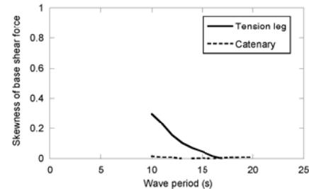
Fig.10 Comparison of skewness of tower base shear force between tension leg system and catenary system
