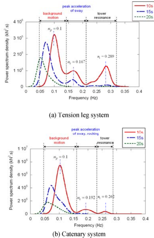
Fig. 9 Comparison of power spectrum density of tower base shear force
