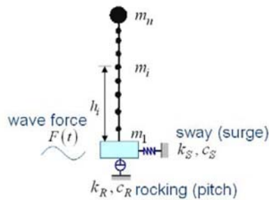
Fig. 2 Sway-rocking model
