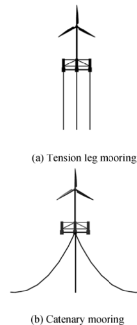
Fig. 1 Types of mooring systems analyzed in this study
