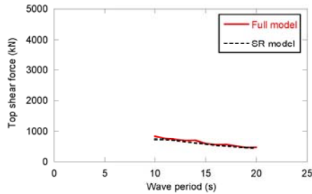
(b) Top shear force
