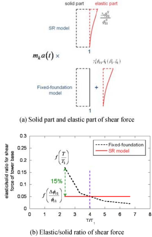
Fig. 7 Comparison of elastic parts of shear force
