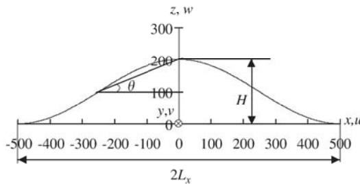
Fig. 7. Cross-section of model at y=0 .
