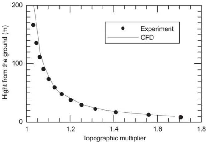
Fig. 1. Comparison of predicted and measured directional topographic multipliers.
