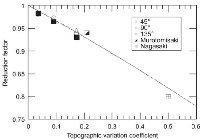
Fig. 10. Variation of reduction factors with topographic variation coefficients.
