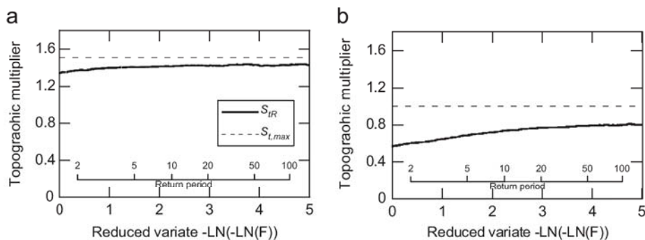
Fig. 6. Topographic multipliers with return period at (a) Murotomi-saki and (b) Nagasaki.
