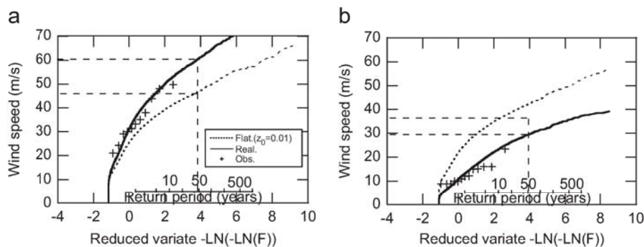
Fig. 4. Extreme wind distributions at the two stations: (a) Murotomisaki and (b) Nagasaki.
