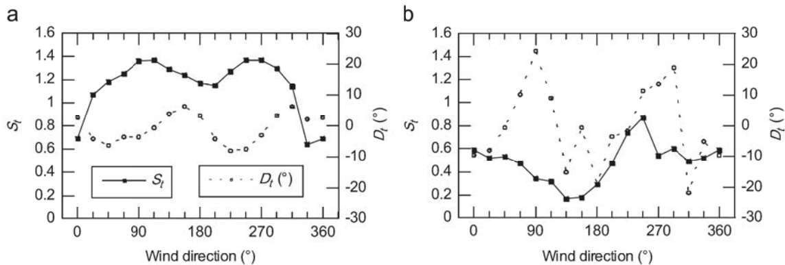
Fig. 3. Directional topographic multipliers S_{ti} and deviations of wind directions D_{ti} at the two stations: (a) Murotomisaki and (b) Nagasaki.
