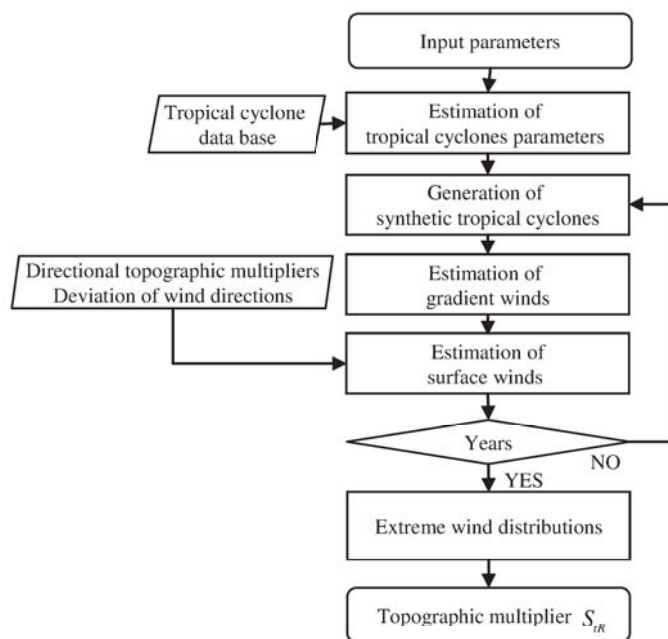
Fig. 5. Flowchart for evaluation of topographic multiplier by MCS, S_{tR} .
