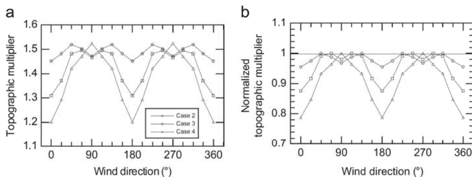
Fig. 8. Variation of (a) directional topographic multipliers and (b) normalized ones with wind directions.
