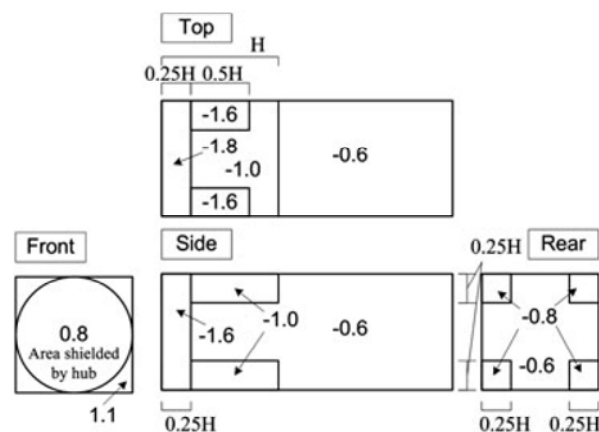
Figure 18. Mean pressure coefficients proposed for DLC6.1 from the wind tunnel test.
