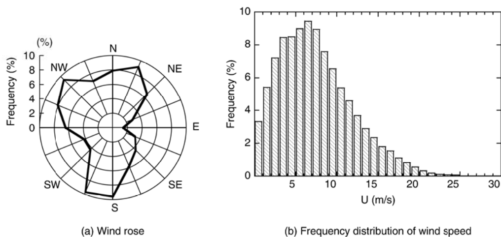
Figure 3: Characteristics of offshore wind conditions.
