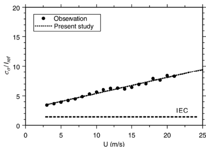
Figure 6: Variation of \sigma_{\sigma}/I_{ref} with wind speed.
