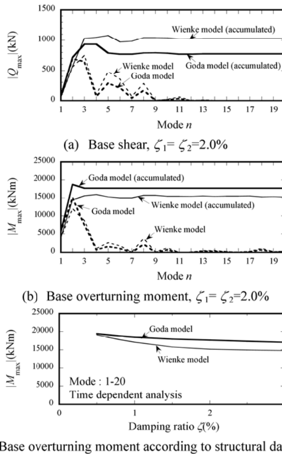
Fig. 5 The maximum section forces by time dependent analysis ( \lambda\eta_c = 1\text{m} )
