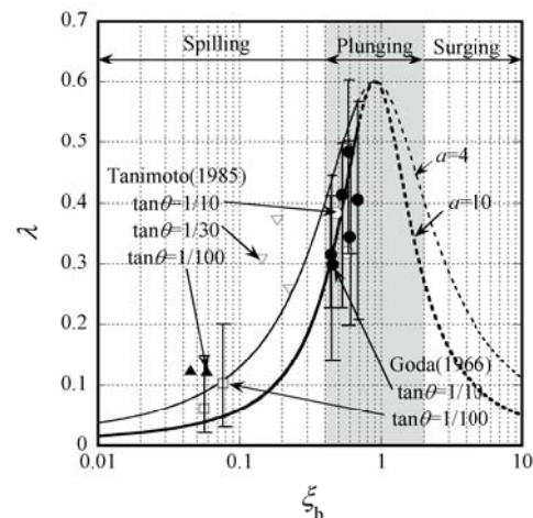
Fig. 7 Relationship between surf similarity parameter \xi_b and curling factor \lambda
