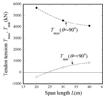
Fig. 10 Tendon tension dependency on L ( D_p:H_p = 6 m: 23 m, T_0 = 2290 kN, under storm conditions).
