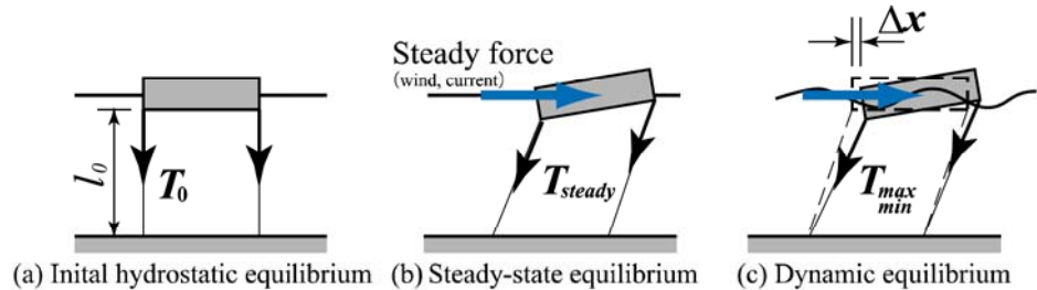
Fig. 3 Definition of tendon tension at each equilibrium state.
