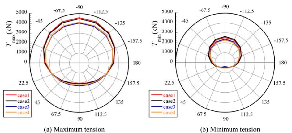
Fig. 6 Tensions in tendon No. 1 for wind direction \theta ( L:D_p:H_p = 30 \text{ m}:6 \text{ m}:23 \text{ m} ; T_0 = 2290 \text{ kN} under storm conditions).
