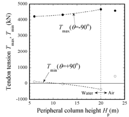
Fig. 9 Tendon tension dependency on H_p ( L:D_p = 30 m: 6 m, T_0 = 2290 kN, under storm conditions).
