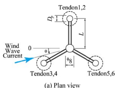
Fig. 2 Parameters used in this study.
