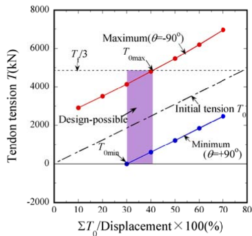
Fig. 7 The maximum and minimum tendon tension dependencies on the initial tension and a design-possible area ( L:D_p:H_p = 30 \text{ m}:6 \text{ m}:23 \text{ m} , tendon No. 1, under storm conditions).
