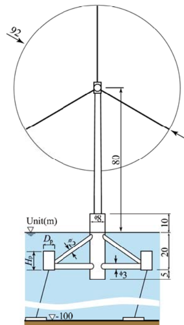
(b) Elevation
