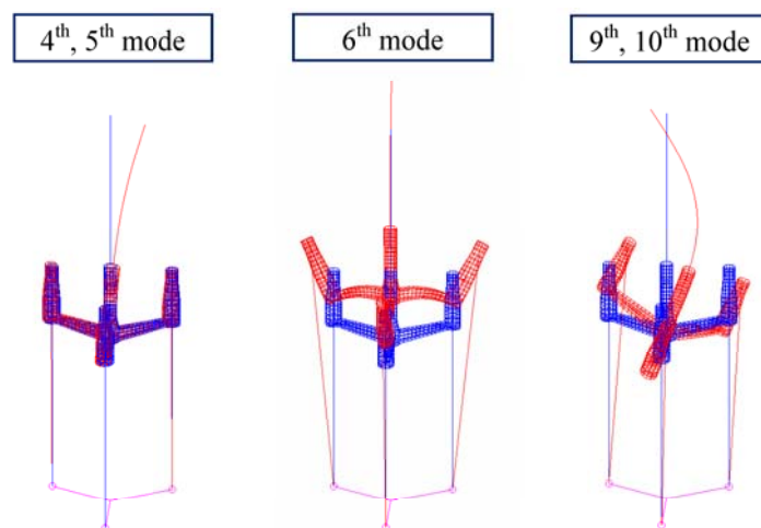
Fig.5 Vibration modes
