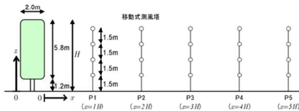
Figure 2 The flow behind a pine tree
