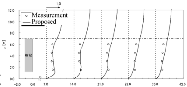
Figure 4. The mean wind speed behind a pine tree
