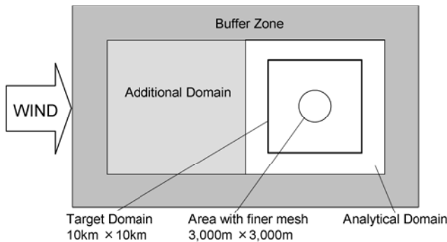
Figure 2. Computational domain
